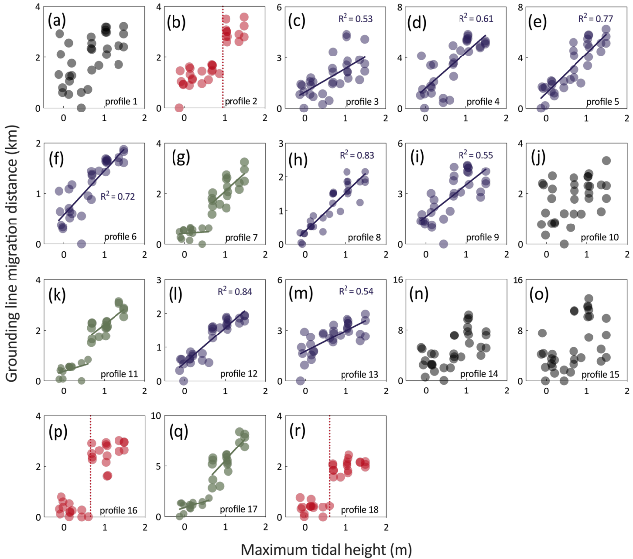
330 Figure 4. Tidal GL migration modes of AmIS. The label in the lower right corner of each subplot indicates the corresponding profile number, consistent with the profile numbering in Figure 1b. The relationship between GL migration distance and maximum tidal height is depicted across different modes: Threshold (subplots with red points represent profiles where a threshold relationship is observed between GL migration and maximum tidal height. The red dashed line indicates the threshold beyond which significant GL migration occurs), Linear (subplots with purple points show a linear relationship between GL migration and maximum tidal height, with the purple solid line representing the best-fit linear regression), Asymmetric (subplots with green points display an asymmetric relationship, with two green solid lines representing the linear fits for different ranges of maximum tidal height), and no clear mode (subplots with black points indicate profiles where no clear mode is observed between GL migration and maximum tidal height). Note that a GL migration distance of 0 km represents the location of the seawardmost GL observed in each profile, which is used as the reference point for calculating relative migration distances.
