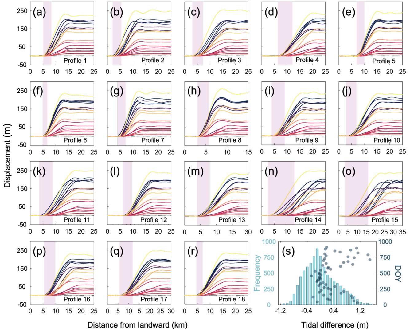
215 Figure 2. (a-r) DROT-derived displacements extracted along 18 profiles located perpendicular to the grounding zone, as shown in Figure 1b. The colour of each line corresponds to the DROT measurement date (yellow is Jan 2021, purple is Nov 2021) (colours consistent with scale used in Figure 1b), and light purple shading indicates the width of the measured GZ. (s) Distribution of tidal difference recorded through the year-long study period (light blue bars), shown alongside tidal difference at times of each SAR image acquisition (grey dots).
