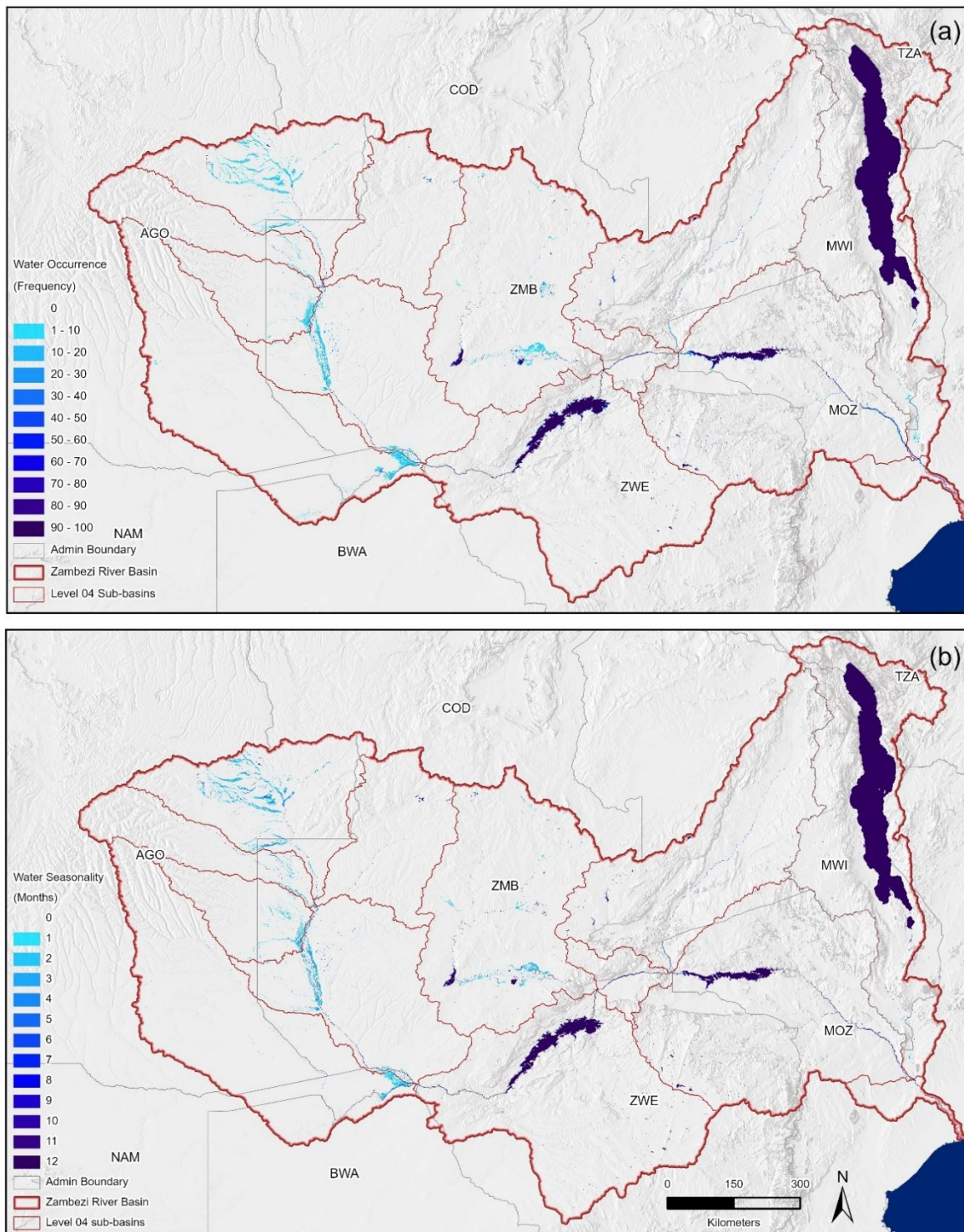
Figure 7. JRC average water (a) occurrence and (b) seasonality (number of months water is present within a year) from Pekel et al. (2016) for the Zambezi basin from 1984–2021
