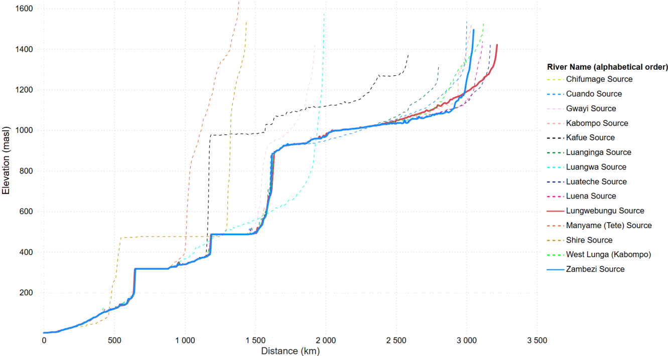
380 Figure 4. Longitudinal profiles of Zambezi River Basin tributaries to the river mouth, derived using ESRI’s Trace Downstream Tool. Steep vertical drops indicate large waterfalls, gorges and reservoir dam walls, while flat horizontal lines indicate large lakes or reservoirs.
