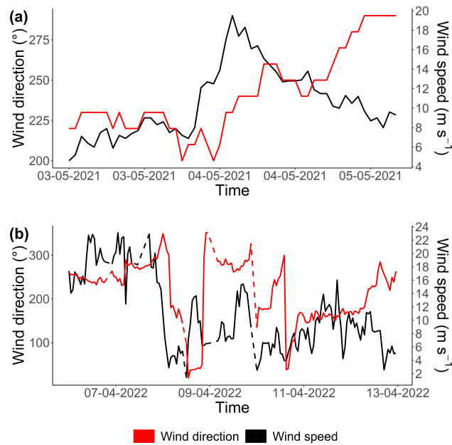
Figure D1. Wind direction (red line, in degrees from true north) and wind speed (black line, in \text{m s}^{-1} ) recorded during the two strong wind events shown in Fig.7: (a) May 2021 and (b) April 2022. Dashed lines indicate gaps in the time series due to missing data.
