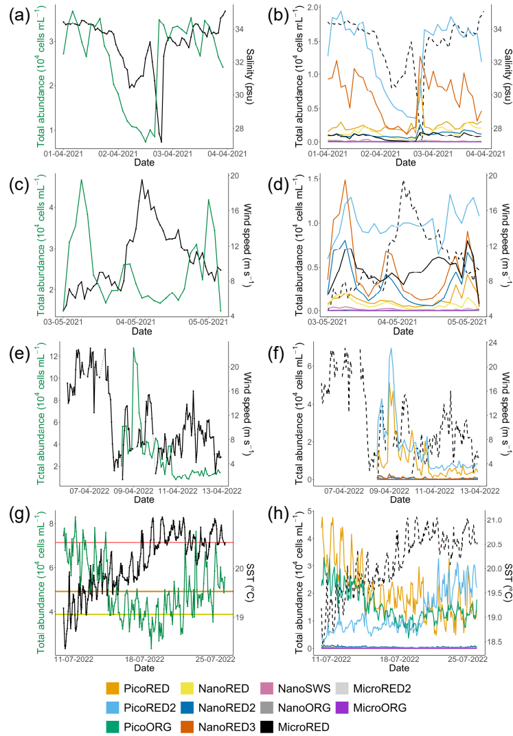
Figure 7. Examples of rare events recorded on MAREL Carnot station during the study: (a,b) a desalination event in April 2021, (c,d) a high wind speed period in May 2021, (e,f) a strong wind period in April 2022 and (g,h) a high SST event (heatwave) in July 2022. Each of the corresponding parameters is shown on the second y -axis (right axis) as a solid black line in the (a,c,e,g) left-hand figures and as a dotted line in the (b,d,f,h) right-hand figures. The absolute total abundance are given in the left-column (a,c,e,g; green line) and the absolute abundance for each phytoplankton group are given in the right-column (b,d,f,h; colored lines). The three horizontal lines of the figure (g) represent the 90 % (yellow), 95 % (orange) and 99 % (red) percentile of the SST observations of the MAREL Carnot station between March 24 th 2004 and September 30 th 2023. The abiotic data (salinity, SST, wind speed) presented here comes from (a,b,e,f,g,h) MAREL Carnot station and (c,d) Météo France (Boulogne-sur-Mer station).
