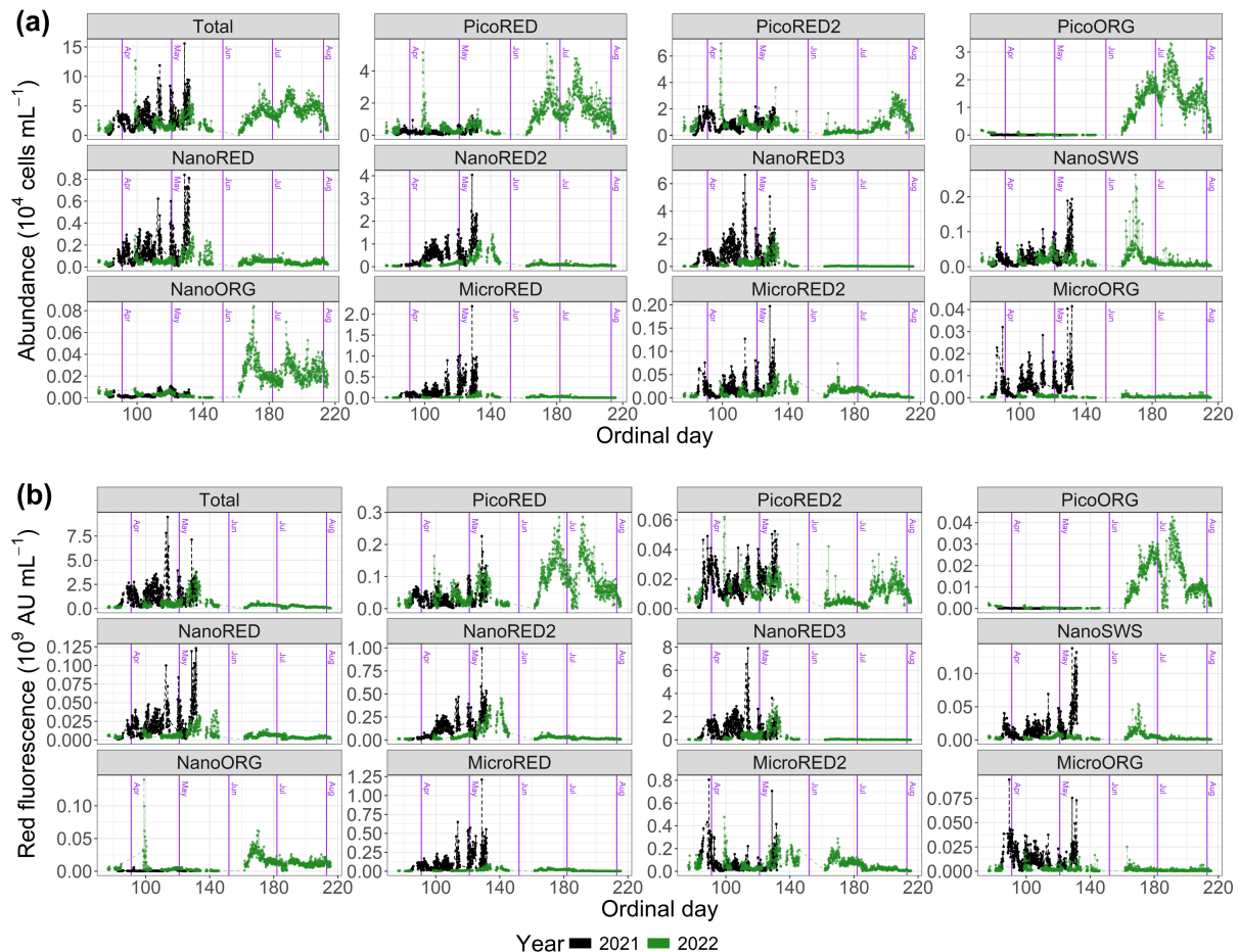
Figure 5. Phytoplankton data recorded with the automated flow cytometer (CytoSub) for each sampled Ordinal day: (a) phytoplankton abundance and (b) phytoplanktonic red fluorescence (proxy of the chlorophyll a expressed in Arbitrary Units per mL; AU). These data are represented in total values and per optically-discriminated PFG. The black line and dots represent 2021 data and the green line and dots represent 2022 data. The purple vertical lines indicate the start of each month.
