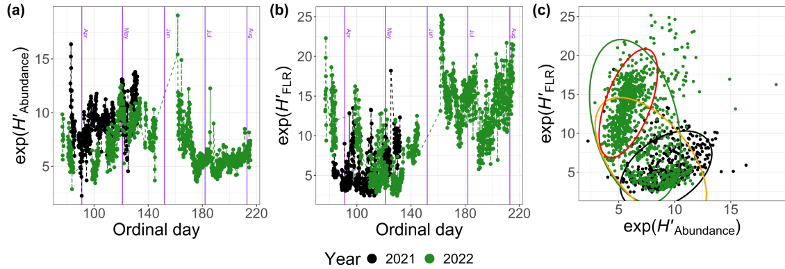
Figure 11. Exponential values of Shannon index H' calculated for 2021 and 2022 based on (a) the abundance ( H'_{Abundance} ) and (b) the FLR ( H'_{FLR} ) in function of the Ordinal day and (c) comparison of these two quantities. The ellipses represent the t distributions with a 95 % confidence interval. The orange ellipse take into account 2022 data before June 9 th and the red one takes into account that after June 9 th .
