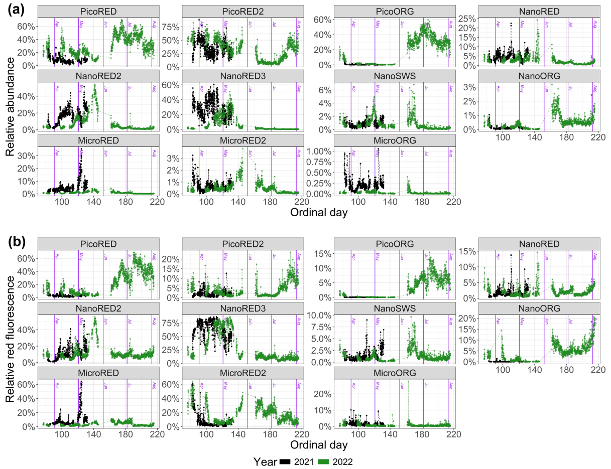
Figure 6. Phytoplankton data recorded for each group with the automated flow cytometer (CytoSub) for each sampled Ordinal day: (a) PFGs relative abundance and (b) PFGs relative red fluorescence (proxy of the chlorophyll a ). The relative values of each group are computed as the ratio of the group's value to the total sum across all groups. The black line and dots represent 2021 data and the green line and dots represent 2022 data. The purple vertical lines indicate the start of each month. Another representation of these results is proposed in Appendix C.
