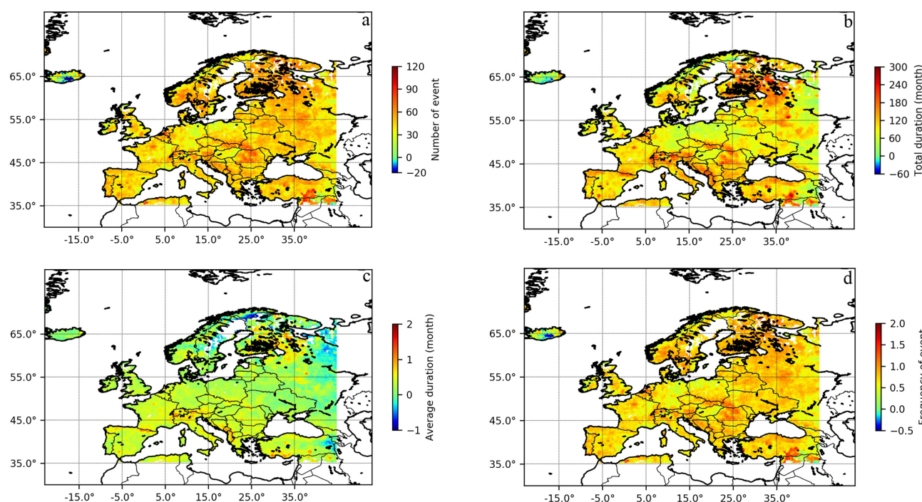
Figure 1. Changes (future-reference periods) in drought characteristics across Europe under SSP5-8.5 based on the median ensemble of the ISIMIP models. a) Changes in the number of drought events, b) changes in total drought duration in month, c) changes in average drought duration in month, and d) changes in frequency.
