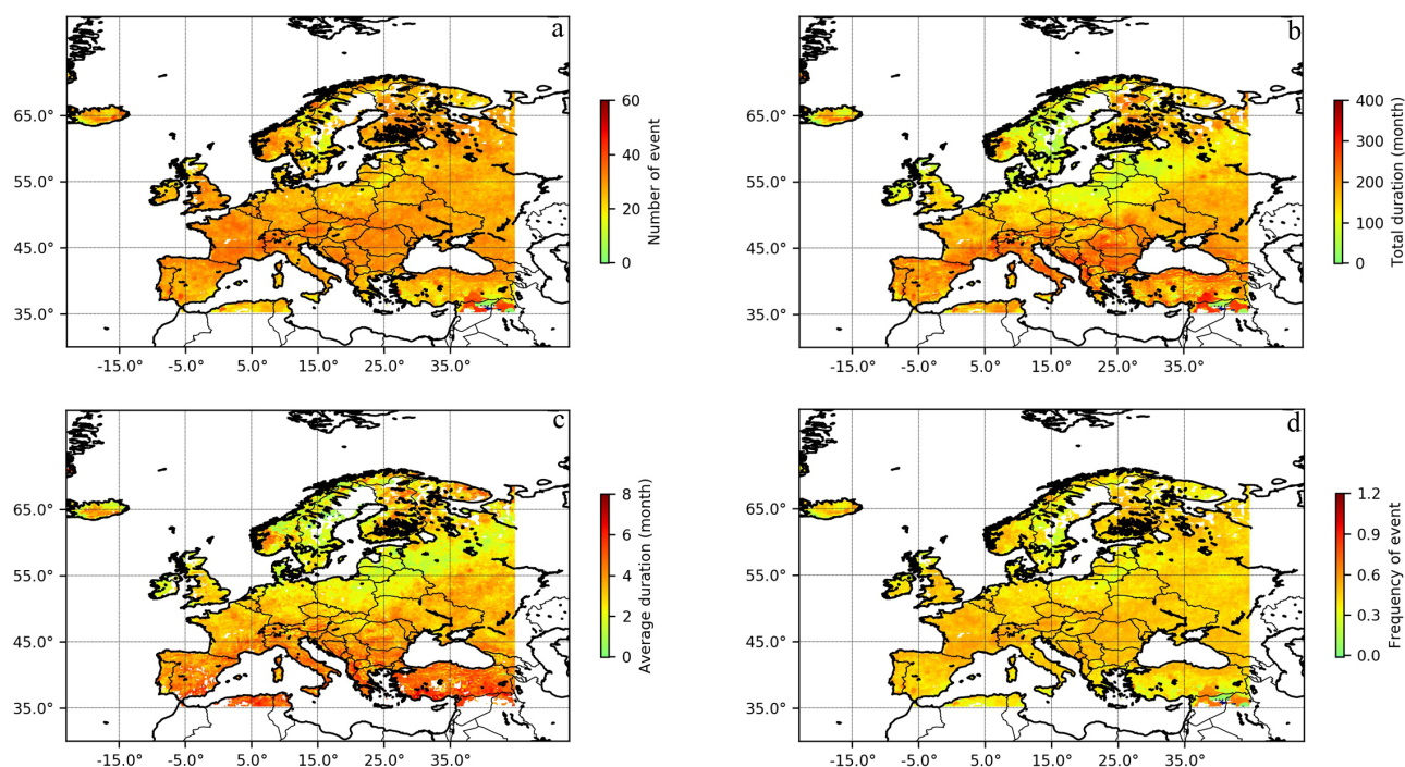
Figure 3. Changes (future-reference periods) in compound event characteristics across Europe under SSP5-8.5 based on the median ensemble of the ISIMIP models. a) Changes in the number of compound events, b) changes in total compound duration in month, c) changes in average compound duration in month, and d) changes in compound frequency.
