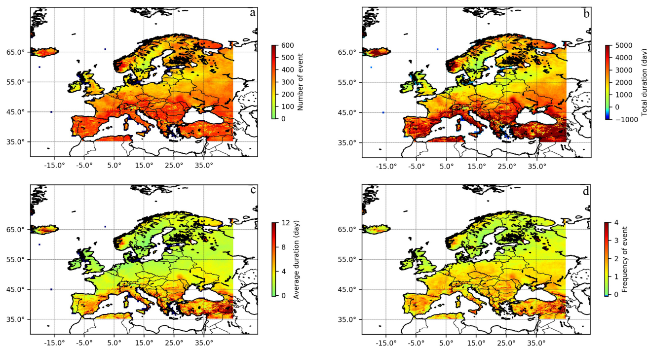
Figure 2. Changes (future-reference periods) in heatwave characteristics across Europe under SSP5-8.5 based on the median ensemble of the ISIMIP models. a) Changes in the number of heatwave events, b) changes in total heatwave duration in day (total number of day for 62 years is 11,408 days), c) changes in average heatwave duration in day, and d) changes in frequency.
