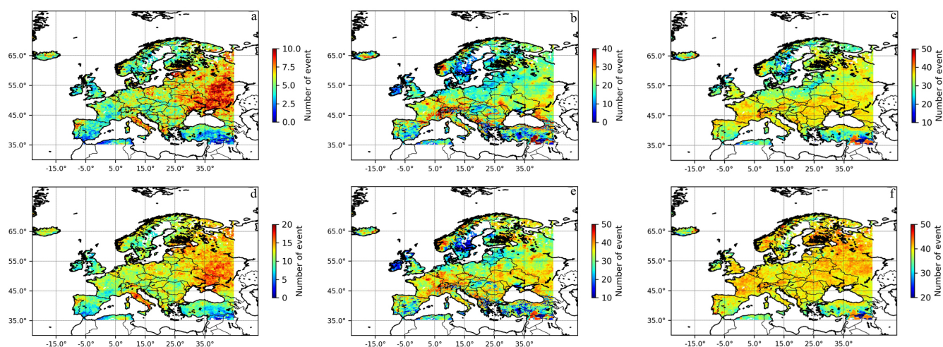
Figure 4. Hotspot regions for compound drought and heatwave (CDH) derived from the number of CDH event across Europe. a) Hotspot regions based on historical period (1953-2014), b) hotspot regions based on future period under SSP1-2.6 (2039-2100), and c) hotspot regions based on future period under SSP5-8.5 (2039-2100). d,e,f) Same as a, b, and c but for cascading drought and heatwave (CaDH). The number of CnC events was obtained from the median ensemble of the ISIMIP models.
