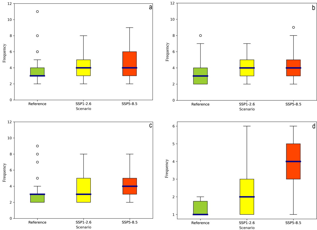
Figure 6. The predictions of drought and heatwave impacts in Germany under reference period (1953-2014) and future period (2039-2100) for SSP1-2.6 and SSP5-8.5. a) Prediction of drought impact on economic sector, b) Prediction of drought impact on non-economic sector, c) Prediction of drought impact on ecosystem sector, and d) Prediction of heatwave impact on humans. The Y axis shows the number of impacts in a year when impacts are predicted from all models. Lower box indicates 25 percentile, middle orange line indicates median, and upper box indicates 75 percentile. The whiskers show the 10 and 90 percentiles. Open circles indicate outliers.
