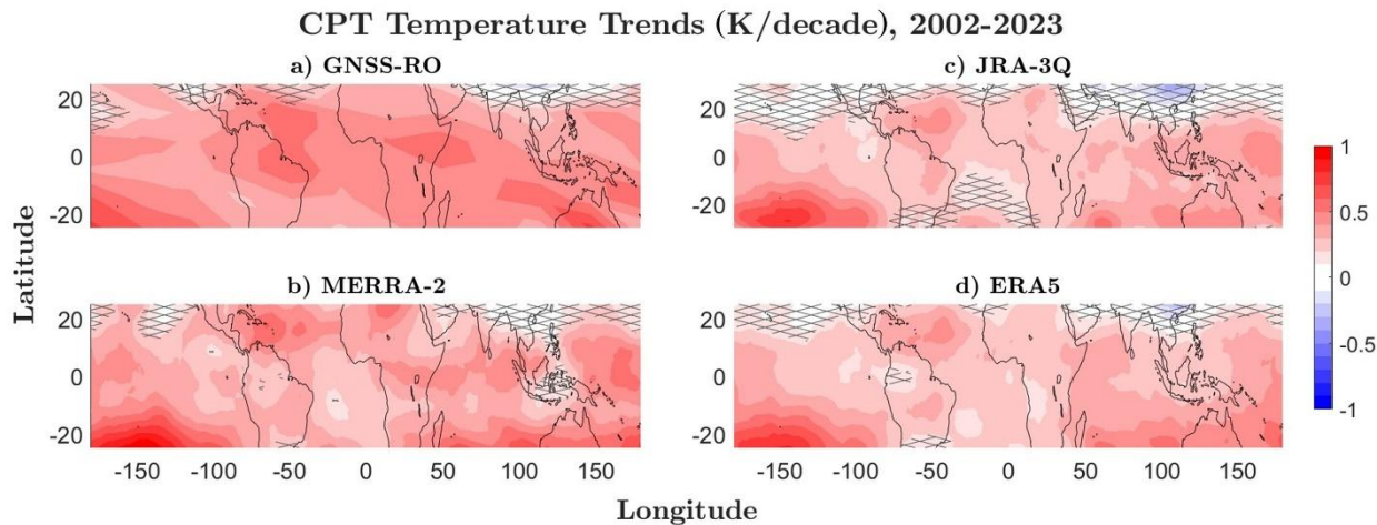
320 Figure 5. Long-term (2002–2023) temperature trends at the cold-point tropopause (CPT) based on (a) GNSS-RO, (b) MERRA-2, (c) JRA-3Q, and (d) ERA5 data. Trends not significant at the 95% confidence level are marked with grey cross-hatching.
