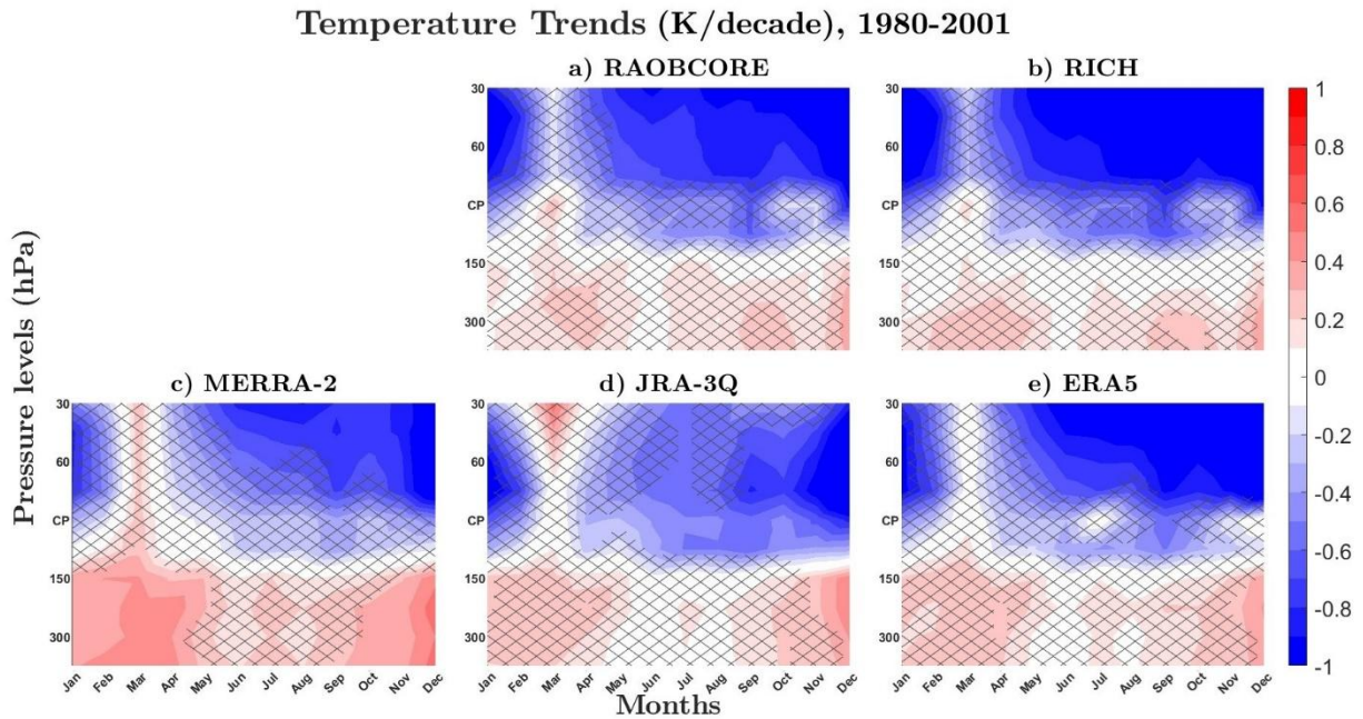
400 Figure 9. The seasonal cycle of long-term temperature trends (1980-2001) at the cold point (CP) and different pressure levels based on (a) RAOBCORE, (b) RICH, (c) MERRA-2, (d) JRA-3Q, and (e) ERA5 data (30°N–30°S). Trends not significant at the 95% confidence level are marked with crosses.
