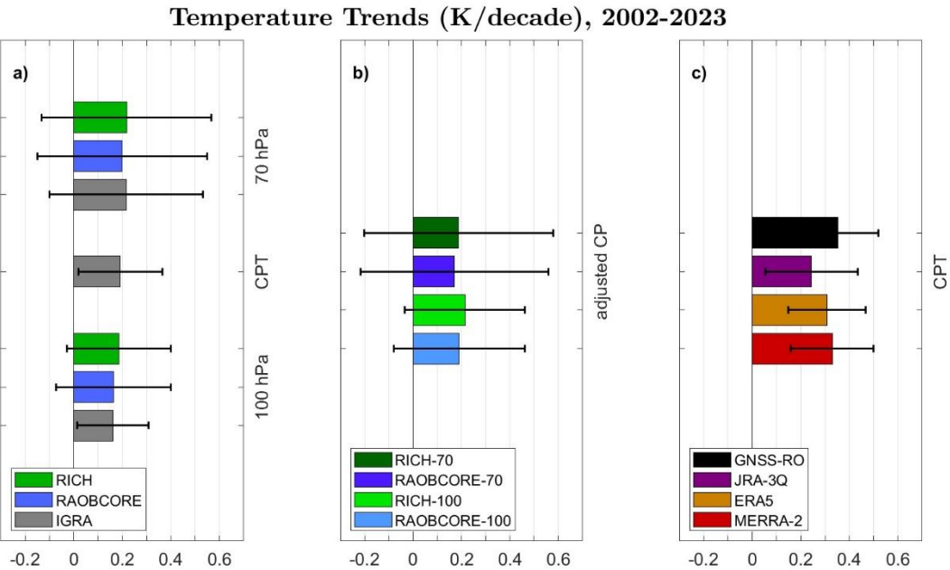
Figure 4. Tropical average (30°S-30°N) temperature trends during 2002-2023 for (a) the cold-point tropopause (CPT) and nearby 295 pressure levels for unadjusted (IGRA) and adjusted (RAOBCORE, RICH) data; (b) the CPT trends based on adjusted data and the Nearby Level approach and (c) the CPT based on GNSS-RO and reanalysis data. Error bars show the \pm 2 sigma confidence intervals of the trend taking into account the adjusted effective sample size.
