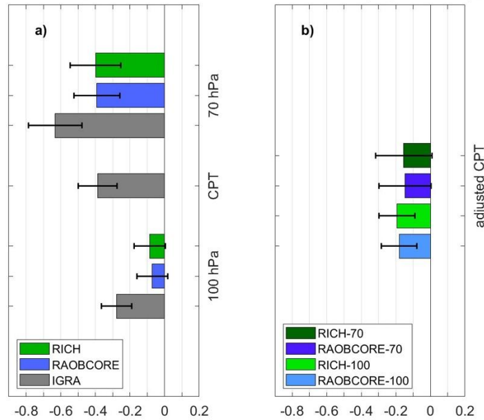
245 Figure 2. Tropical average (30°S-30°N) temperature trends during 1980-2023 for (a) the cold-point tropopause (CPT) and nearby pressure levels for unadjusted (IGRA) and adjusted (RAOBCORE, RICH) data and (b) for the CPT trends based on adjusted data and the Nearby Level approach. Error bars show the \pm 2 sigma confidence intervals of the trend taking into account the adjusted effective sample size.
