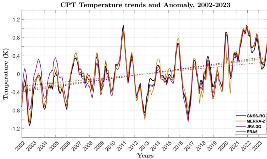
265 Figure 3. Tropical mean (30°S–30°N) deseasonalized cold-point tropopause (CPT) temperature anomalies and the linear trend based on the GNSS-RO, MERRA-2, JRA-3Q, and ERA5 data. The data are smoothed over 5 months for visibility.
