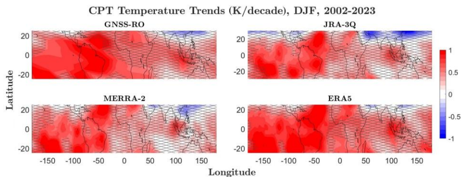
Figure A4. Same as the Figure 5 but for DJF.
