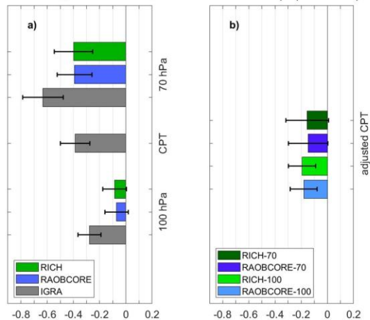
Figure 2. Tropical average (30°S-30°N) temperature trends during 1980-2023 for (a) the cold-point tropopause (CPT) and nearby pressure levels for unadjusted (IGRA) and adjusted (RAOB CORE, RICH) data and (b) for the CPT trends based on adjusted data and the Nearby Level approach. Error bars show the \pm 2 sigma confidence intervals of the trend taking into account the adjusted effective sample size.
