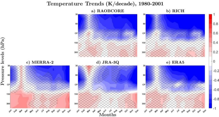
Figure 9. The seasonal cycle of long-term temperature trends (1980-2001) at the cold point (CP) and different pressure levels based on (a) RAOBCORE, (b) RICH, (c) MERRA-2, (d) JRA-3Q, and (e) ERA5 data (30°N–30°S). Trends not significant at the 95% confidence level are marked with hatches or crosses.
