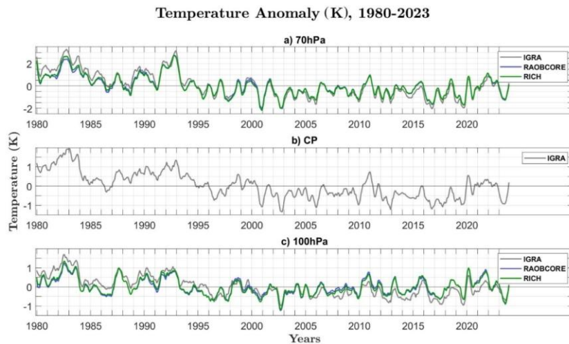
Figure 1. Tropical mean (30°S-30°N) deseasonalized temperature anomalies from 1980 to 2023 for (a) 70 hPa, (b) the cold-point tropopause (CPT), and (c) 100 hPa levels, using IGRA (gray), RAOB CORE (blue), and RICH (green) datasets. The data are smoothed over 5 months for visibility.
