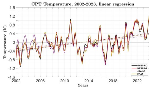
Figure A2. Same as Figure 3 but based on a simple conventional linear regression with constant and linear term only
