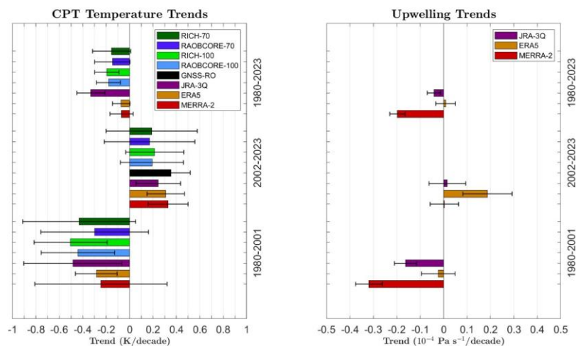
Figure 10. Tropical average (30°S-30°N) of trends in cold-point tropopause (CPT) temperature and tropical upwelling based on different observational and reanalysis datasets for the three time periods: 1980-2001, 2002-2023, and 1980-2023. The reanalysis tropical upwelling is the vertical residual circulation averaged over 100 and 70 hPa. Error bars show the \pm 2 sigma confidence intervals of the trend taking into account adjusted effective sample size.
