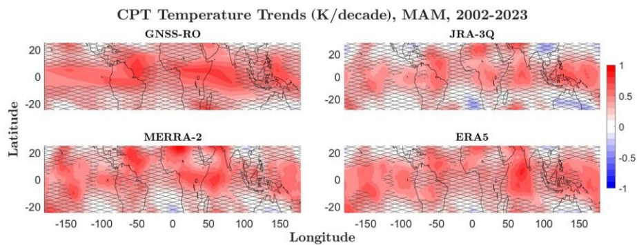
Figure A5. Same as the Figure 5 but for MAM.
