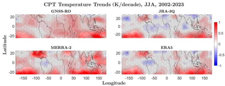
Figure A6. Same as the Figure 5 but for JJA.
