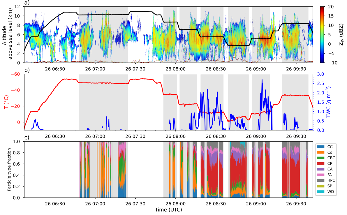
Figure 2. Time height measurements conducted by the Falcon 20 during IOP7a. a) RASTA W-band radar reflectivity observation and aircraft altitude ( reflectivity values within \pm 300 m of the aircraft are interpolated ). b) Temperature and total water content (TWC) estimated using by the method of Fontaine et al. (2014). c) Time series (10 seconds averaged) showing the fraction of hydrometeor types with D > 300 \mu\text{m} classified as Capped columns (CC), Columns and needles (Co), Combination of bullets or columns (CBC), Compact particles (CP), Complex assemblages of planes, columns, or dendrites (CA), Fragile aggregates (FA), Hexagonal planar crystals (HPC), splintered particles (SP), and Water drops (WD) following the method developed by Jaffaux et al. (2022).
