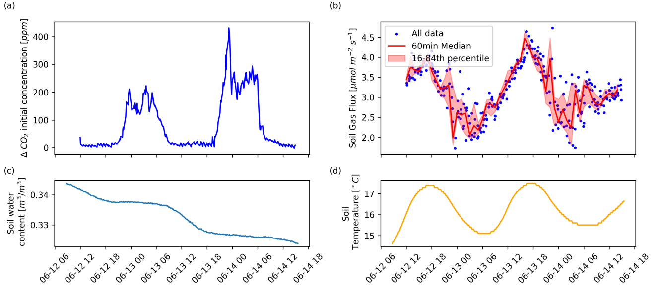
Figure 7. Field measurement of the low-cost soil gas flux system for two day period where it shows (a) initial concentration of CO_2 at each measurement, (b) the soil gas flux of CO_2 with median of the moving window of 60 minutes, (c) the top soil water content and (d) the top soil temperature.
