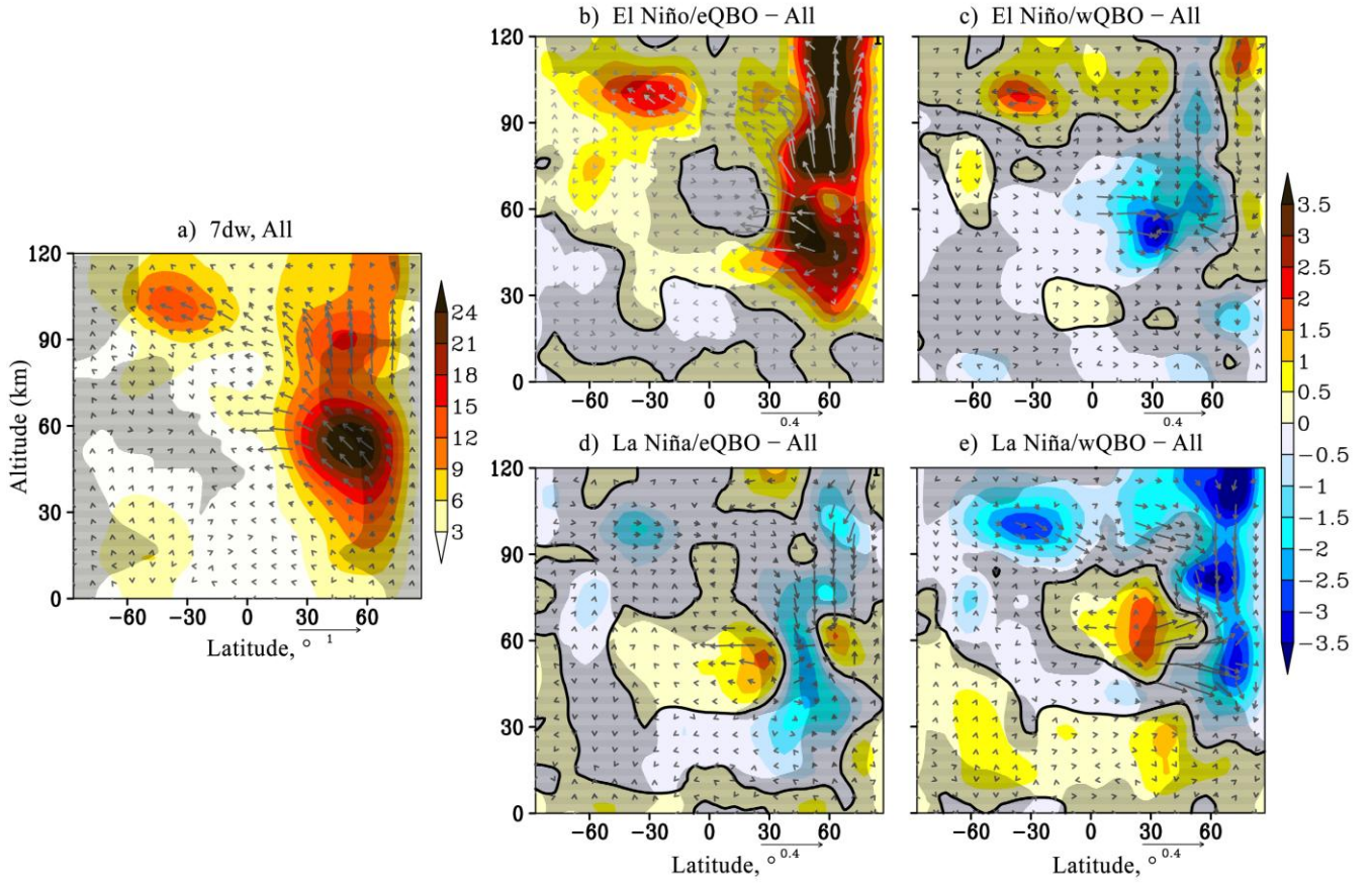
300 Figure 5: The same as Fig. 1 but for the westward travelling atmospheric NM with \tau = 7 days, m = 2 .
