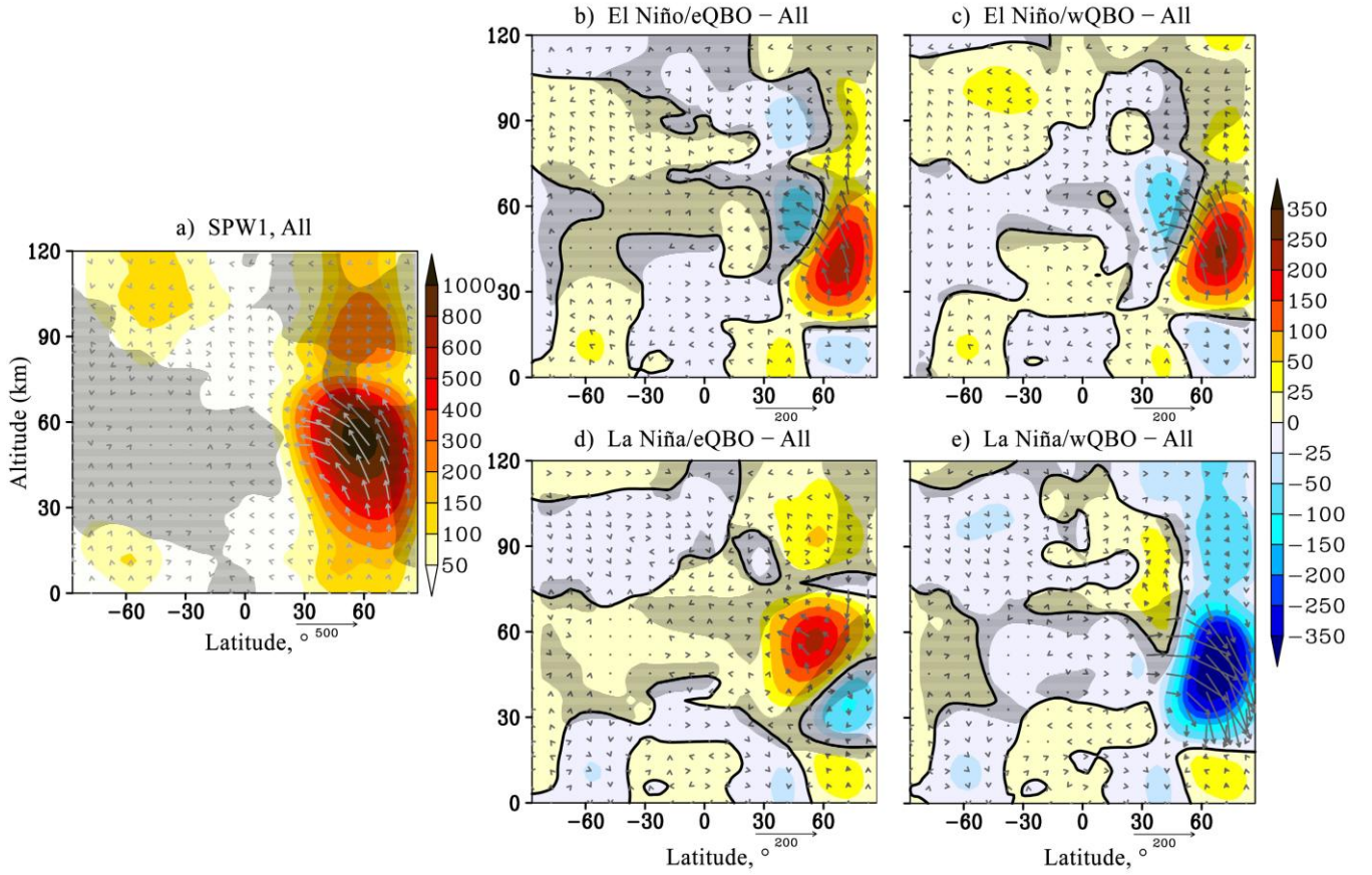
235 Figure 1. a): amplitude of the geopotential height variations caused by SPW1 (gp.m, shaded), EP flux ( m^2/s^2 , arrows). Hatched areas show negative refractive index beyond the waveguide. Data is averaged over January–February and all MUAM simulations; b-e): respective amplitude and EP flux increments due to change of ENSO/QBO phase, hatched areas show insignificant data at 95%. Vertical EP flux component is multiplied by 200.
