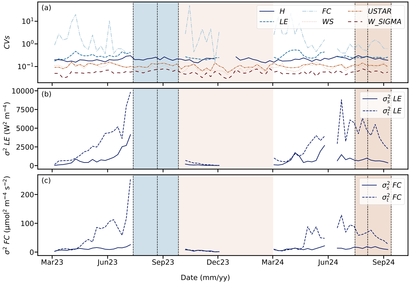
Figure 6. (a) Coefficients of variation (CVs), calculated after Oren et al. (2006), for FC , LE and H , \bar{u} , USTAR , and W\_SIGMA (logarithmic scale); (b) spatial ( \sigma_s^2 LE ) and temporal ( \sigma_t^2 LE ) variance for LE ; (c) spatial ( \sigma_s^2 FC ) and temporal ( \sigma_t^2 FC ) variance for FC . The plotted values are weekly means calculated at 30-min temporal resolution from the flux time series. Vertical dashed lines represent, from left to right, the harvest dates of the crops in 2023, for rapeseed (13 July 2023), barley (22 August 2023) and corn (26 September 2023); and in 2024, for rapeseed (15 July 2024), barley (5 August 2024) and corn (13 September 2024). Dashed areas correspond to the 2023 harvest period (dull blue), the winter period (dull yellow) and the 2024 harvest period (dull brown), for a better comparison with Figure 5. Due to the two very long gaps in AF1 and AF3 (see Fig. 4), plus some shorter gaps, there were no data corresponding to the harvest period in 2023 for FC or LE and only few weeks of data in the winter period. Note the logarithmic scale in panel (a), introduced due to the large magnitude of some of the CVs of FC for visualization purposes. No gap-filled data were used to create this plot.
