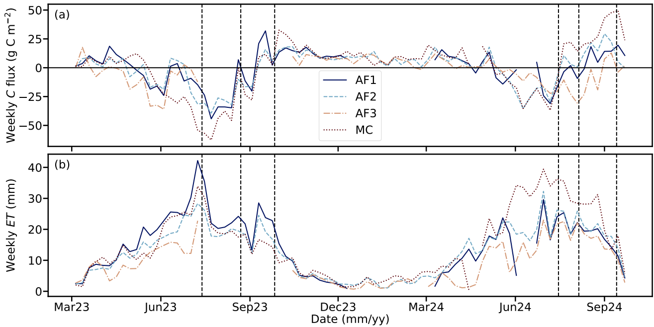
Figure 4. Weekly sums of the net ecosystem carbon exchange as a carbon (C) flux (a) and evapotranspiration (b, ET ) measured at the four stations, across the measurement campaign. Sums were calculated from the gap-filled time series. Missing values correspond to gaps longer than 2 weeks, which were not considered in the analysis. The horizontal line in sub-plot (a) highlights the zero line, separating the uptake (negative fluxes) from the emission (positive fluxes). Vertical dashed lines represent, from left to right, the harvest dates of rapeseed (13 July 2023), barley (22 August 2023) and corn (26 September 2023) in 2023; and rapeseed (15 July 2024), barley (5 August 2024) and corn (13 September 2024). Due to the requirement of taking only gap-filled data for gaps up to two weeks of duration, there were some missing weeks for all stations and two very long gaps, in summer 2023 for AF3 and in winter 2023/24 for AF1.
