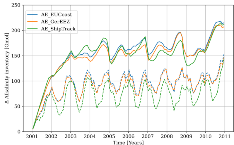
Figure 2: The excess alkalinity inventory across the entire model domain, integrated over the entire water column (solid lines) and over the upper mixed layer (dashed lines).
