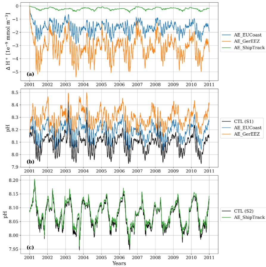
435 Figure 12: (a) Time series of H^+ changes resulting from the OAE implementations. For the AE_EUCoast and AE_GerEEZ scenarios, the time series is taken at location S1, as marked in Figs. 11(a) and (b). For the AE_ShipTrack scenario, the time series is taken at location S2, as marked in Fig. 11(c). (b) Time series of pH at location S1 with and without OAE perturbation. (c) Time series of pH at location S2 with and without OAE perturbation.
