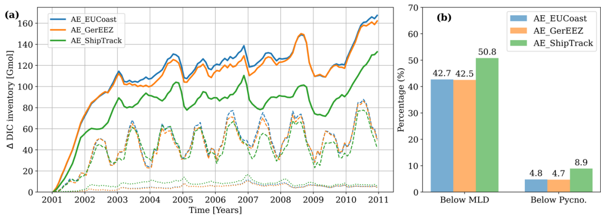
385 Figure 9: (a) The excess DIC inventory across the entire model domain, integrated over the entire water column (solid lines), below the upper mixed layer (dashed lines) and below the permanent pycnocline (dotted lines). (b) the percentage of the total excess DIC inventory below the mixed layer depth (Below MLD) and below the permanent pycnocline (Below Pycno.). The calculation is based on the model results of 2006-2010.
