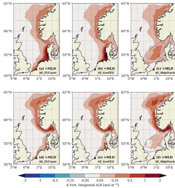
Figure 3: Difference of vertically integrated alkalinity between the OAE scenarios and the CTL simulation over the upper mixed layer (a-c) and below the mixed layer (d-f) in the last simulation year (2010). Black dotted lines outline the OAE sites. Note the nonlinear color bar.
