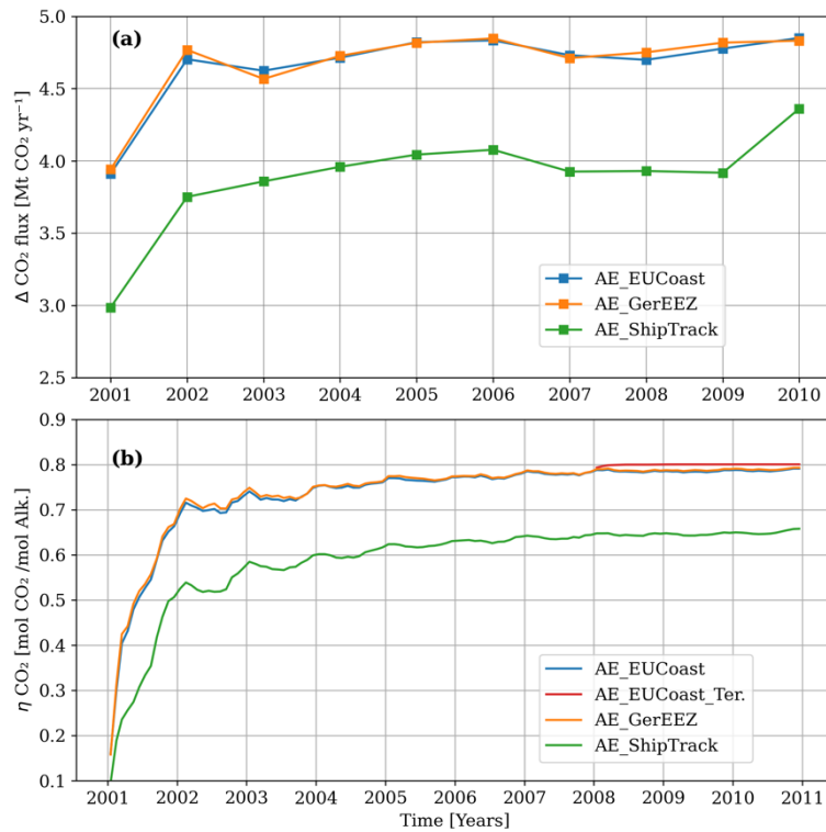
355 Figure 7: (a) The yearly excess \text{CO}_2 uptake over the model domain due to OAE in different scenarios. (b) The \text{CO}_2 uptake efficiency ( \eta \text{CO}_2 ) with a unit of mol \text{CO}_2 uptake per mol alkalinity addition, defined as the accumulated \text{CO}_2 uptake relative to the accumulated alkalinity addition.
