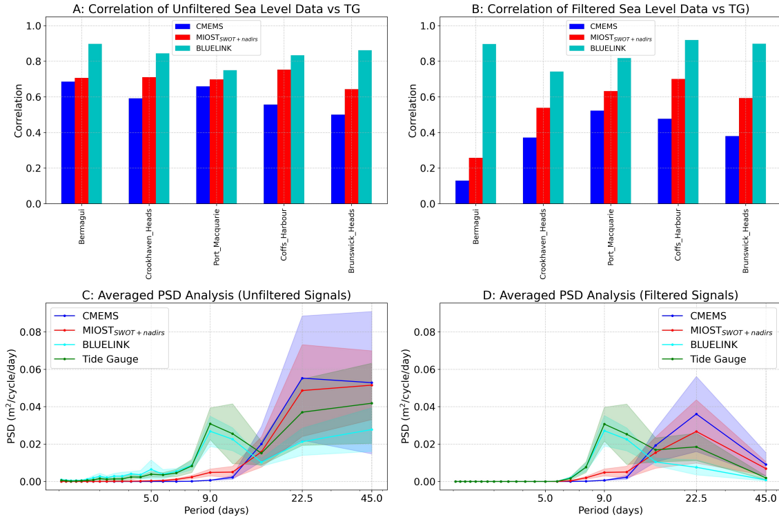
Figure 3. Upper panels: Correlation of CMEMS, MIOST SWOT+ nadirs and BLUELINK time series with the TG data at the closest grid point to each in-situ station. The plot shows the correlation considering unfiltered (A) and filtered (B) time series. Lower panels: The averaged PSD of the same time series as above in their unfiltered (C) and filtered (D) version. The shaded areas represent the standard deviation across these gauges at each period.
