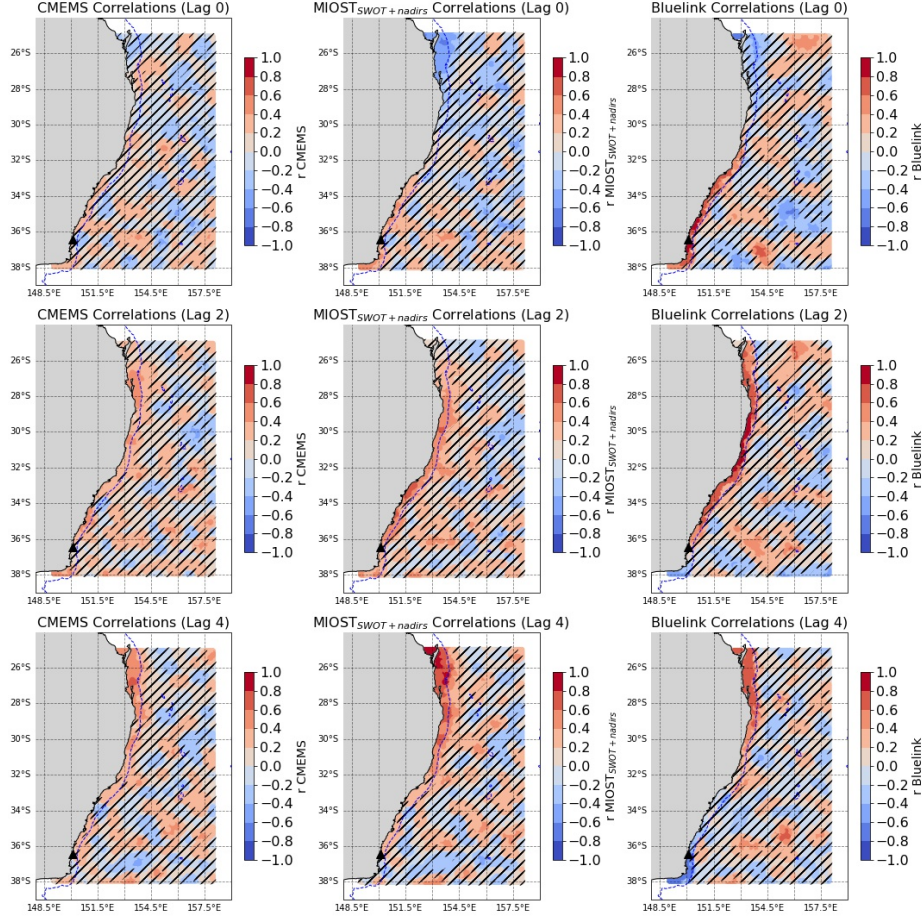
Figure 4. Correlation coefficient ( r ) of filtered CMEMS, MIOST SWOT+nadirs and BLUELINK time series at each grid point against the filtered TG data of the station Bermagui (black triangle). Each row corresponds to the lag correlation at day 0, 2, 4. The bathymetry contour of -500m is shown to identify the shelf break. Locations where the correlation is not statistically significant are marked with black diagonal stripes.
