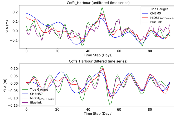
Figure 2. Daily sea level data from CMEMS, MIOST SWOT+nadirs , BLUELINK and the Coffs_Harbour tide gauge. The upper plot shows the full signals, while the lower plot is obtained by filtering out components longer than 29 days (0.035 cycles per day in frequency) and shorter than 7 days (0.15 cycles per day in frequency).
