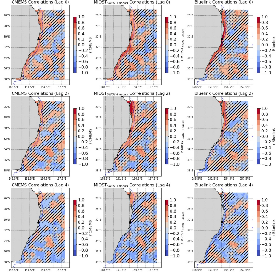
Figure B2. Correlation coefficient ( r ) of filtered CMEMS, MIOST SWOT+nadirs and BLUELINK time series at each grid point against the filtered TG data of the station Coffs_Harbour ((black triangle). Each row corresponds to the lag correlation at day 0, 2, 4. The bathymetry contour of -500m is shown to identify the shelf break.
