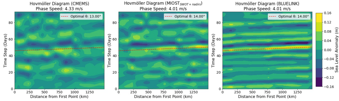
Figure 5. Hovmöller diagrams of CMEMS, MIOST SWOT+ nadirs and BLUELINK filtered time series. Each column represents the sea level anomaly time series at a coastal location within the parallelogram shown in Figure 1, progressing from the southwesternmost point northward along the coast. The dotted lines correspond to the best estimate of the westward propagation speed (see Section 3.3). The x-axis represents the distance from the southwesternmost point along the coastline.
