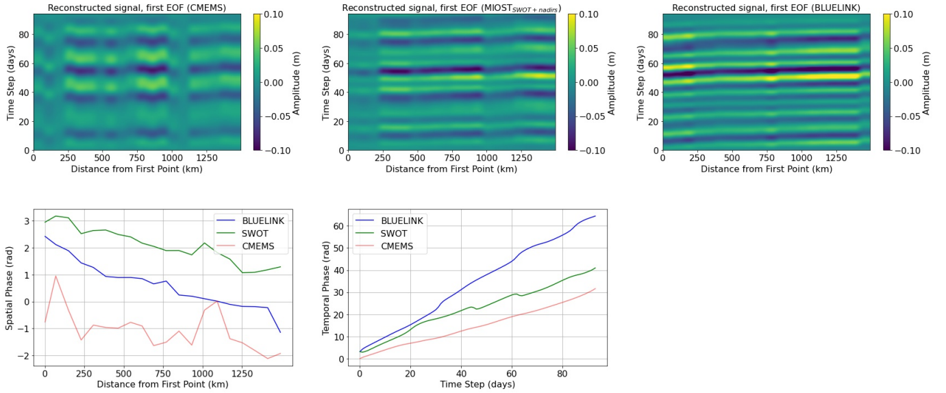
Figure 6. Upper plots: Hovmöller diagrams showing the amplitude of the reconstructed signal from the first CEOF for CMEMS, MIOST SWOT+nadirs and BLUELINK. Each column represents the reconstructed sea level anomaly time series at a coastal location within the parallelogram shown in Figure 1, progressing from the southwesternmost point northward along the coast. Lower plots: Spatial (left) and temporal (right) phase of the first CEOF.
