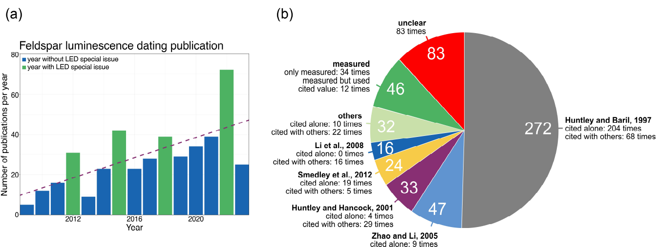
135 Figure 1: Summary of the literature review. a) amount of published literature, covering the topic of dose rate determination for feldspar luminescence dating, per year from 2009 until 2023. Green bars represent years after a LED in which a LED special issue was published. The purple dashed line shows the trend of publication numbers per year over time. b) references given for used K- concentrations in the analysed 432 studies. The white numbers within the diagram show the total citation numbers. Note that the total sum exceeds the sum of 432 studies analysed since some studies cited several references. The “unclear” section is the sum of studies who did not cite or mention a K-concentration, studies mentioning a value for the K-concentration without a reference, and studies vaguely giving information.
