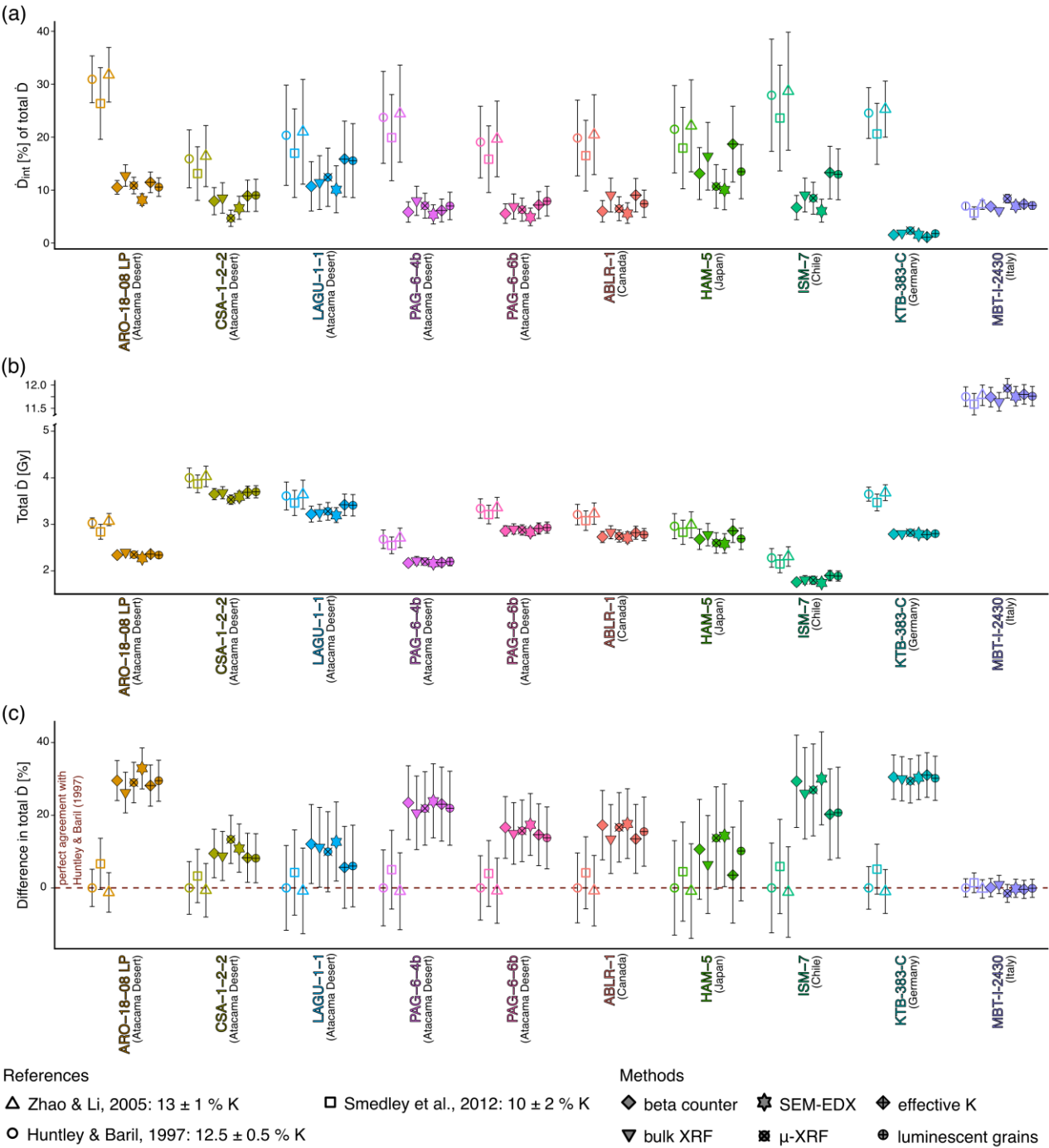
565 Figure 4: \dot{D} results, with \dot{D}_{\text{int}} and total \dot{D} calculated with DRAC (Durcan et al., 2015) based on the different K-concentrations of the three most cited literature values (open symbols), the measured K-concentrations (filled symbols), and luminescence-weighted K estimates (filled symbols). All other input variables are described in section 3.5. a) the proportion of the \dot{D}_{\text{int}} in the corresponding total \dot{D} . b) the total \dot{D} . c) a comparison between the total \dot{D} based on the K-concentration of 12.5 \pm 0.5 (Huntley & Baril, 1997) and
