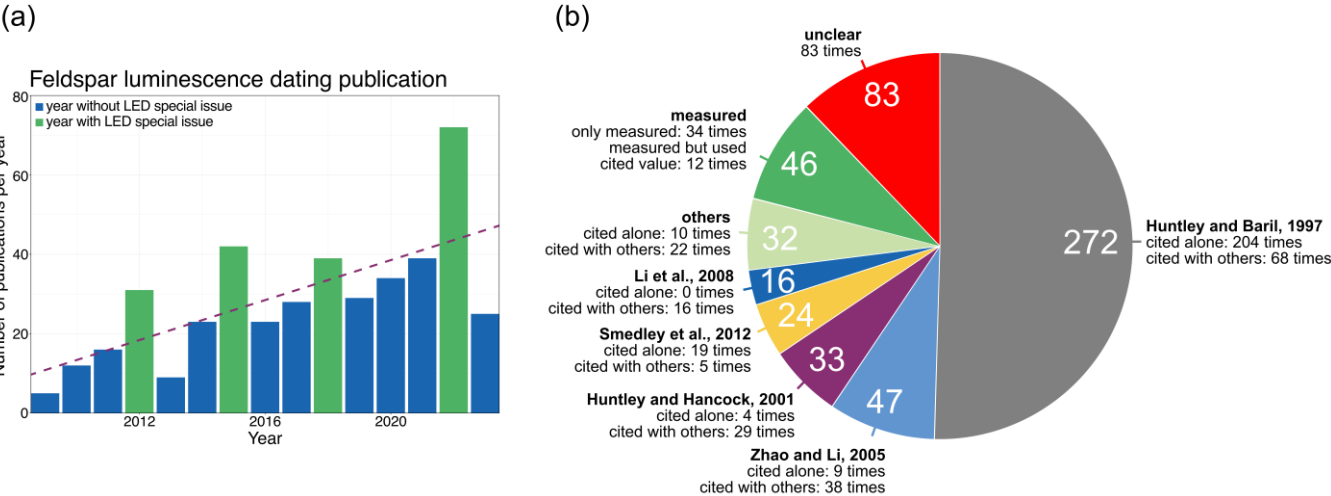
135 Figure 1: Summary of the literature review. a) amount of published literature, covering the topic of dose rate determination for feldspar luminescence dating, per year from 2009 until 2023. Green bars represent years after a LED in which a LED special issue was published. The purple dashed line shows the trend of publication numbers per year over time. b) references given for used K- concentrations in the analysed 432 studies. The white numbers within the diagram show the total citation numbers. Note that the total sum exceeds the sum of 432 studies analysed since some studies cited several references. The “unclear” section is the sum of 140 studies who did not cite or mention a K-concentration, studies mentioning a value for the K-concentration without a reference, and studies vaguely giving information.
