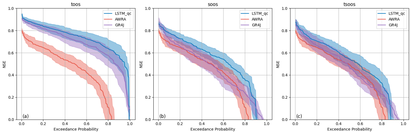
730 Figure A3. Exceedance probability curves of NSE TooS, SooS, and TSooS experiments. Shaded regions show 95% confidence intervals from 1000 block bootstrap replicates (365-day blocks), confirming the robustness of LSTM-QC performance relative to AWRA-L and GR4J.
