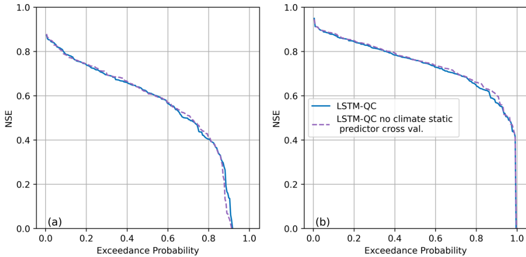
390 Figure 6. Impact of cross-validation on model performance with (right) and without (left) fine-tuning of recalculated quasi-static climatic variables for each fold in TooS validation
