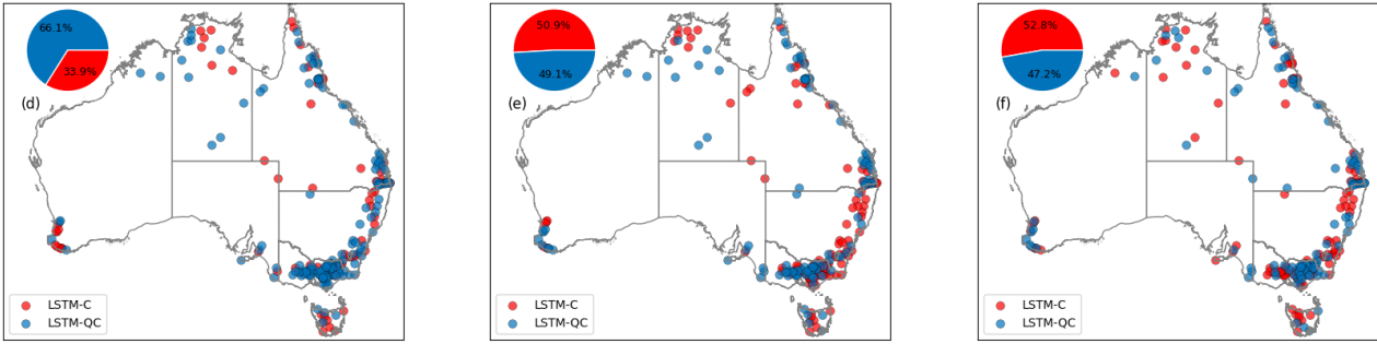
380 Figure 5. Exceedance curve of NSE difference between LSTM-QC, which uses both AWRA-L Q_{tot} and climate dynamic predictors, with LSTM-C, which uses only climate dynamic predictors, illustrating the information gain from including AWRA-L Q_{tot} . Top row shows exceedance probability curves of the NSE difference between LSTM-QC and LSTM-C under TooS (a) SooS (b) and TSooS (c) experiments. Bottom row shows spatial distribution of the best-performing model under each.
