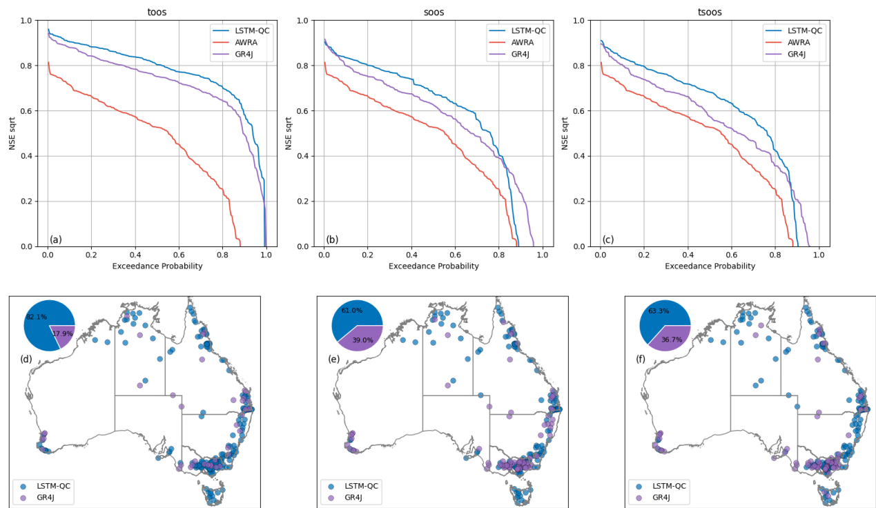
Figure A1. Benchmarking LSTM-QC results against AWRA and GR4J. Top row is exceedance curve of NSE_{sqrt} across all catchments; bottom row shows which model performs best for each catchment. The columns from left to right show TooS, SooS, and TSooS cross-validation experiments
