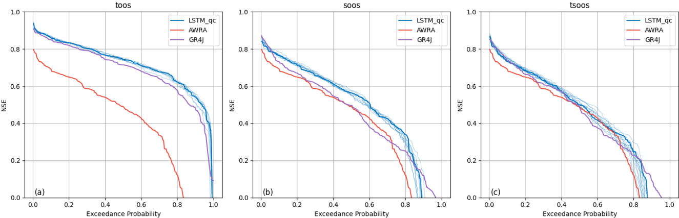
740 Figure A4. NSE exceedance curves from TooS, SooS, and TSooS experiments. Thick blue line shows performance of median timeseries, and lighter blue lines show results from 10 independent LSTM runs with different random seeds.
