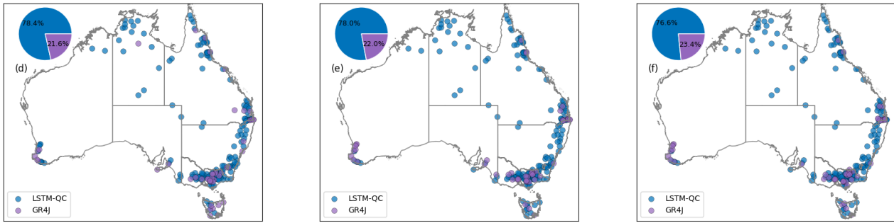
720 Figure A2. Benchmarking LSTM-QC results against AWRA and GR4J. Top row is exceedance curve of Absolute bias across all catchments; bottom row shows which model performs best for each catchment. The columns from left to right show TooS, SooS, and TSooS cross-validation experiments
