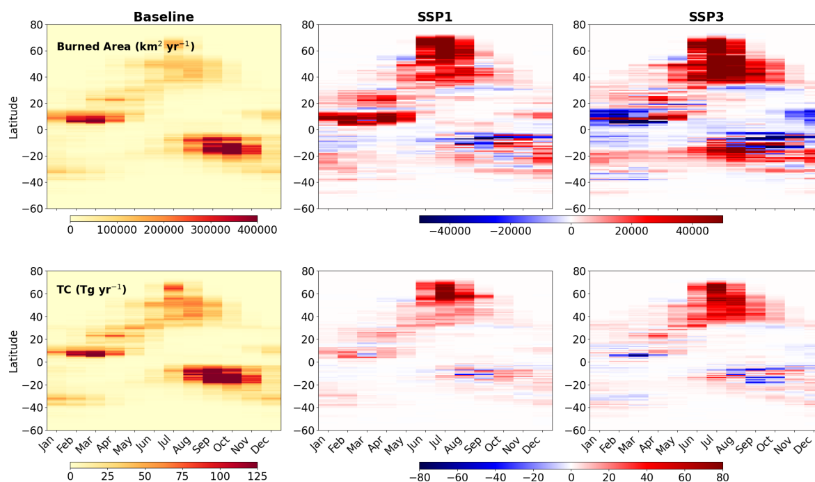
Figure 6. Latitudinal monthly variations in burned area and total carbon emissions at baseline (2015-2024 average) and their future (2090-2099 average) differences in SSP1 and SSP3.
