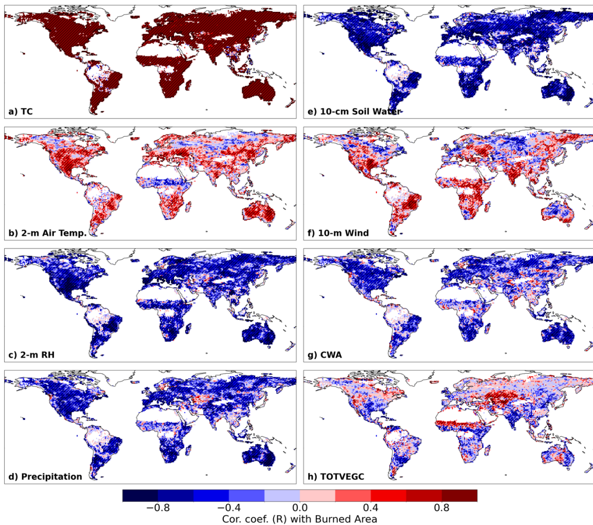
Figure 5. Pearson correlation ( R ) on annual mean monthly time series data (2015 to 2100) between detrended burned area (BA) and (a) TC, (b-g) meteorological variables (2-m surface temperature, 2-m relative humidity (RH), precipitation, 10-cm soil water, 10-m wind velocity, and climate water availability (CWA = precipitation – evapotranspiration)), and (h) total vegetation carbon (TOTVEGC) under SSP1 scenario. Hatch lines are shown over Only regions with a 95% significance level are shown .
