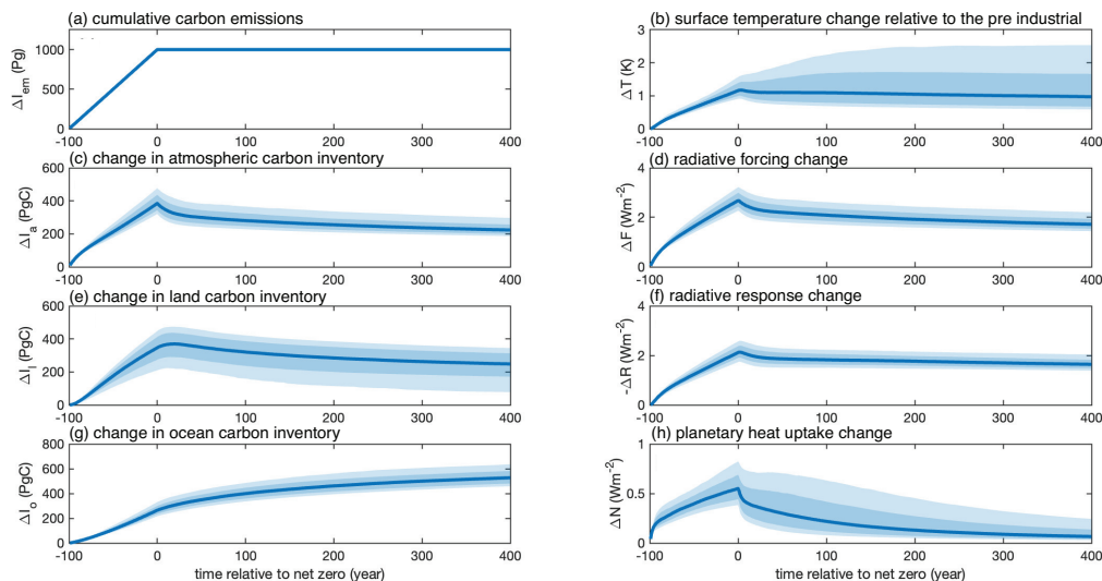
Figure A1. Temporal evolution of carbon and climate variables relative to the time of net zero (years) for the flat10 experiment from the WASP simulations: (a) cumulative carbon emissions, \Delta I_{em}(t') (PgC); (b) surface temperature change relative to the pre industrial, \Delta T(t') (K); (c, e and g) the change in atmospheric carbon inventory, \Delta I_A(t') , land carbon inventory, \Delta I_L(t') and ocean carbon inventory, \Delta I_O(t') , (all in PgC); and (d, f and h) the change in radiative forcing, \Delta F(t') , radiative response, -\Delta R(t') , and planetary heat uptake, \Delta N(t') (all in \text{W m}^{-2} ).
