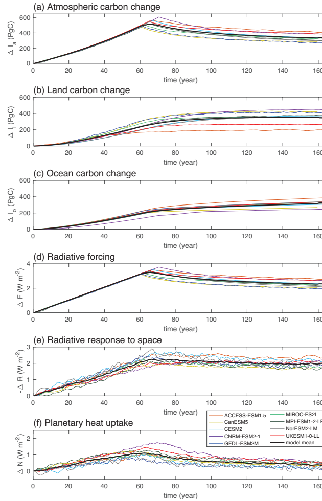
Figure 2. Climate response during emissions and post emissions versus time (year) since the pre industrial for the 9 Earth system models: changes in (a) atmospheric carbon inventory, \Delta I_A (PgC); (b) land carbon inventory, \Delta I_L (PgC); (c) ocean carbon inventory, \Delta I_O (PgC); (d) radiative forcing supplying heat to the climate system, F ( \text{W m}^{-2} ); (e) radiative response representing a heat loss to space, -\Delta R ( \text{W m}^{-2} ); and (f) planetary heat uptake, \Delta N ( \text{W m}^{-2} ), positive representing a gain in heat. The plot includes smoothing of planetary heat uptake with a 10 year running mean.
