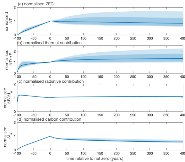
Figure 9. Normalised ZEC and its components following the flat10 experiment from the WASP simulations: (a) the normalised ZEC from the normalised surface temperature change, \Delta T(t') , including the median (line), 1-sigma range (dark shading) and 95% range (light shading); (b) the thermal contribution from the normalised dependence of surface temperature on radiative forcing, \Delta T(t')/\Delta F(t') ; (c) the radiative contribution from the normalised dependence of radiative forcing on atmospheric carbon, \Delta F(t')/\Delta I_A(t') ; and (d) the carbon contribution from the normalised atmospheric carbon, \Delta I_A(t') . In each case, the normalisation is by the value of the variable at the time of net zero.
