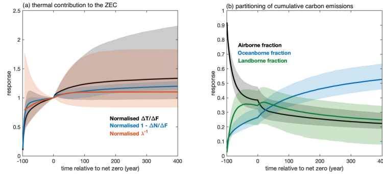
Figure 10. Temporal evolution of thermal and carbon variables affecting the normalised ZEC for the flat10 experiment from the WASP simulations: (a) thermal contribution to the normalised ZEC from the normalised temperature dependence on radiation, \Delta T(t')/\Delta F(t') (black line for median, grey shading for 95% range), normalised fraction of radiative forcing escaping to space, \Delta R(t')/\Delta F(t') = (1 - \Delta N(t')/\Delta F(t')) (blue line and shading) and normalised inverse climate feedback parameter \lambda(t')^{-1} (orange line and pale shading); and (b) the partitioning of cumulative carbon emissions into the airborne fraction (black line for median and grey shading for 95% range), oceanborne fraction (blue line and shading) and landborne fraction (green line and shading) for time (year) relative to net zero.
