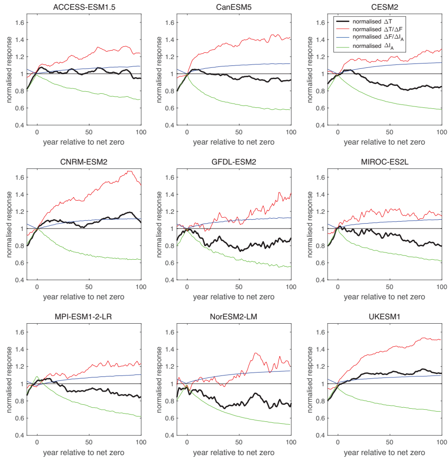
Figure 4. Temporal evolution of the normalised ZEC, the normalised surface temperature change, and its contributions for 9 different Earth system models: the normalised surface temperature change, \Delta T(t') , (black line); the thermal contribution from the normalised dependence of surface temperature on radiative forcing, \Delta T(t')/\Delta F(t') (red line); the radiative contribution from the normalised dependence of radiative forcing on atmospheric carbon, \Delta F(t')/\Delta I_A(t') (blue line); and carbon contribution from the normalised atmospheric carbon, \Delta I_A(t') (green line). The plot includes smoothing of temperature, the alignment of the time series and normalisation as in Fig. 3.
