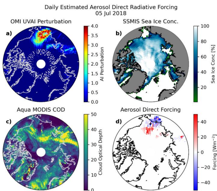
Figure 10. Estimated forcings from aerosol using forcing efficiency slopes and intercepts for 5 July 2018. a) Daily averaged perturbed OMI UVAI. b) SSMIS sea ice concentration (SIC). c) Daily L3 Aqua MODIS COD. d) Estimated aerosol direct radiative forcing (ADRF) for 5 July 2018 based on the OMI UVAI and the look-up table (LUT) of aerosol forcing regressions under different viewing geometry, surface, and cloud conditions.
