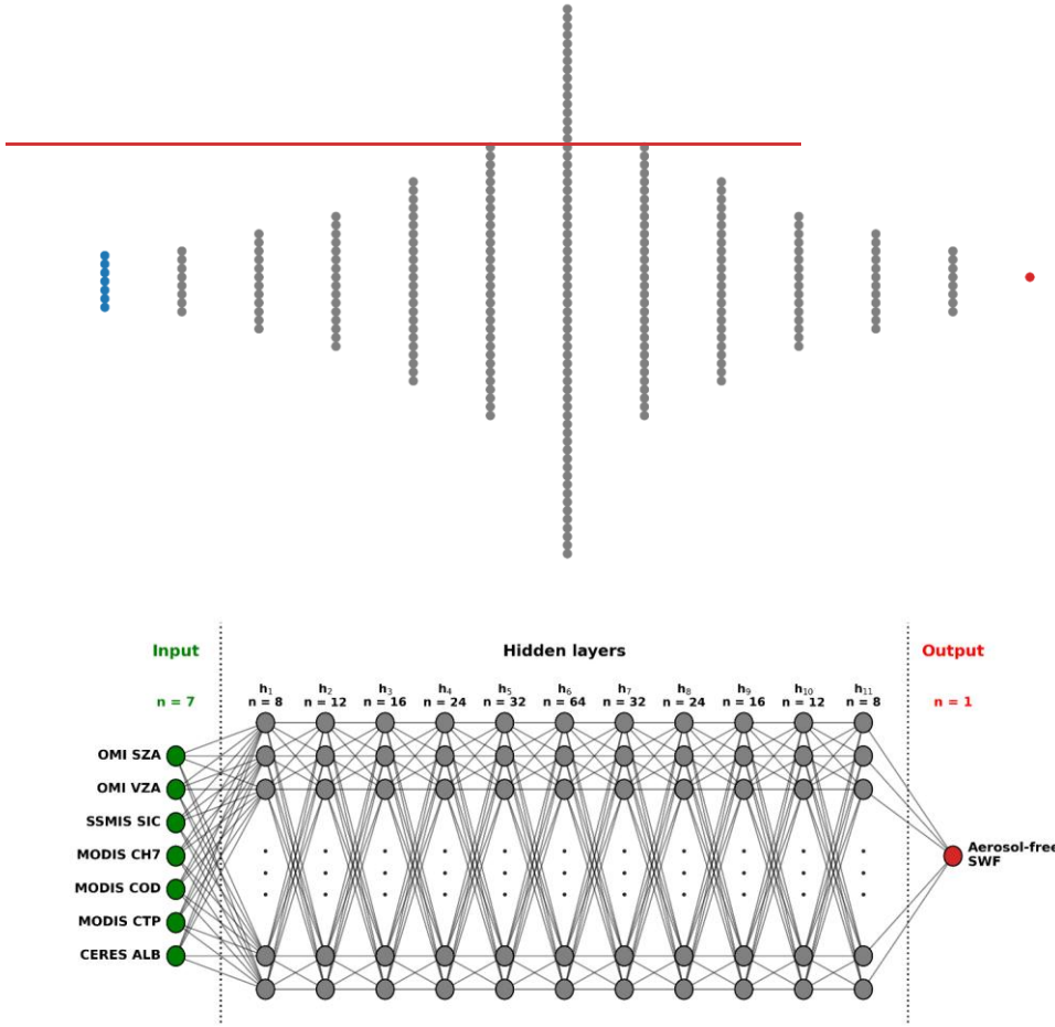
355 Figure 5. Architecture of the neural network for estimating L2 aerosol-free SWF from L2 input values of solar zenith angle (SZA), viewing zenith angle (VZA), sea ice concentration (SIC), cloud optical depth, 2.1 \mu\text{m} reflectance (CH7), cloud optical depth (COD), cloud top pressure (CTP), and surface albedo (ALB). Green circles represent nodes in the input layer, gray circles represent nodes in the hidden layers, and the red circle represents the node in the output layer. While no connections are shown here, all nodes 360 between each layer are fully connected to the next layer in the neural network are fully connected to the nodes in the next layer, as illustrated by the lines connecting the circles.
