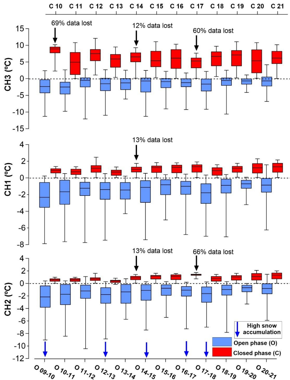
Figure S54. Box-plot of open (blue) and closed (red) phases in A294 between 2010 and 2021. The lost data corresponds to recording failures in the sensors failures due to low battery power .
