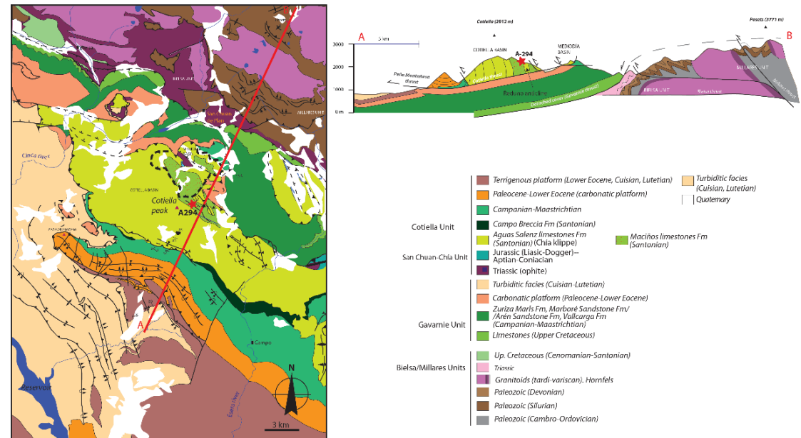
Figure S1: Simplified geological map of the Cotiella area based on IGME Bielsa (179) Ríos et al., (1982) and Campo (212) Robador- Moreno et al., (1999) and López-Mir et al., (2015), and cross-section (along the red line on the map). Red start in the cross-section indicates the location of the A294 ice cave.
