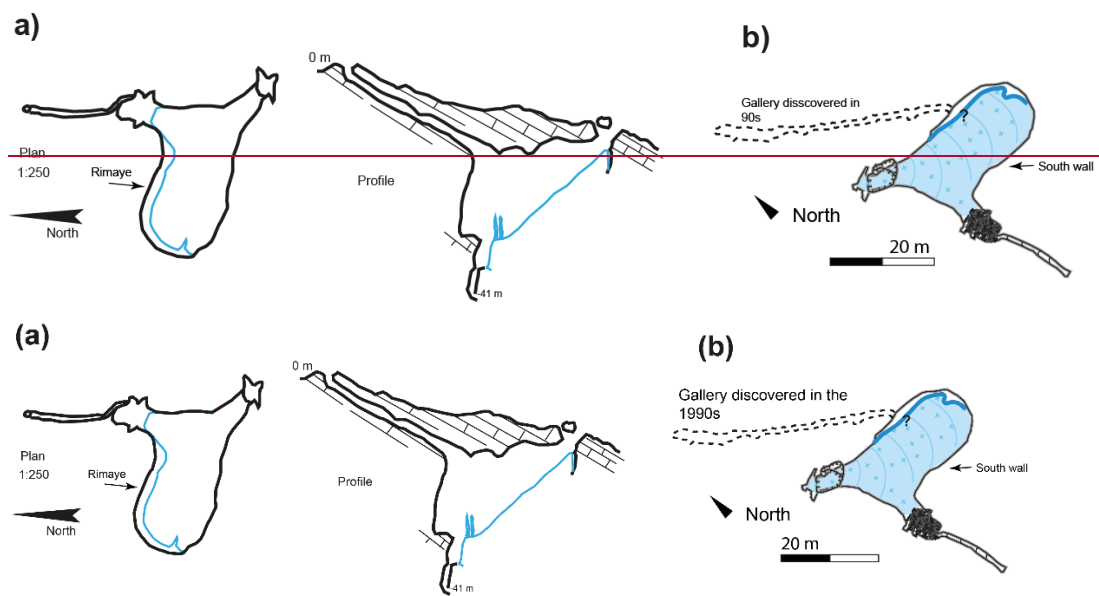
Figure S2. a) A294 cave topography in 1978 digitalized from a map of the Grupo de Espeleología Cataluña Aragón (G.E.C.A). b) Corrected North arrow orientation and topography, and probable extension of the rimaye in that year.
