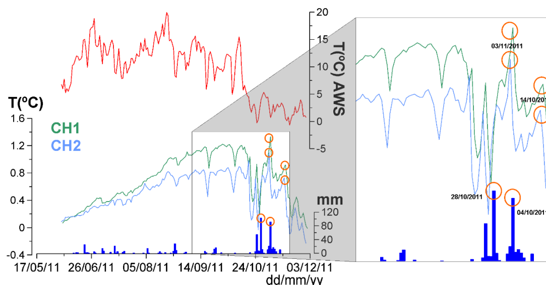
Figure S65. Example of extreme rainfalls (>80 mm) recorded by the Armeña Weather station and delayed increases in cave air temperatures in A294. Red line is the external temperature, while green and blue lines represent the cave temperature variations recorded by the CH1 and CH2 sensors, respectively. Dark blue vertical bars represent precipitation events.
