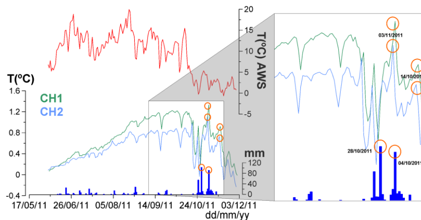
Figure S65. Example of extreme rainfalls (>80 mm) recorded by the Armeña Weather-weather sStation and delayed increases in cave air temperatures in A294. Red line is the external temperature, while green and blue lines represent the cave temperature variations recorded by the CH1 and CH2 sensors, respectively. Dark blue vertical bars represent precipitation events.
