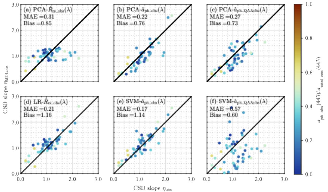
Figure 5. Validation results of the developed models. Comparison between measured ( \eta_{obs} ) and model-estimated \eta values ( \eta_{MDLobs} ) with respect to the fractional contribution of a_{ph,obs}(443) to a_{total,obs}(443) . Upper (a–c) and lower panels (d–f) show CSD models developed by PCA- and ML-based approaches, respectively. Panels (c) and (f) show the results of the same CSD models in panels (b) and (e) but using \hat{a}_{ph,QAA,obs}(\lambda) , whereas panels (b) and (c) use \hat{a}_{ph,obs}(\lambda) determined from in situ observations. MAE denotes the median absolute error.
