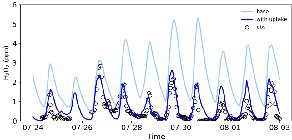
Figure 6. Observed and modelled H 2 O 2 concentrations from 24 July to 3 August.
