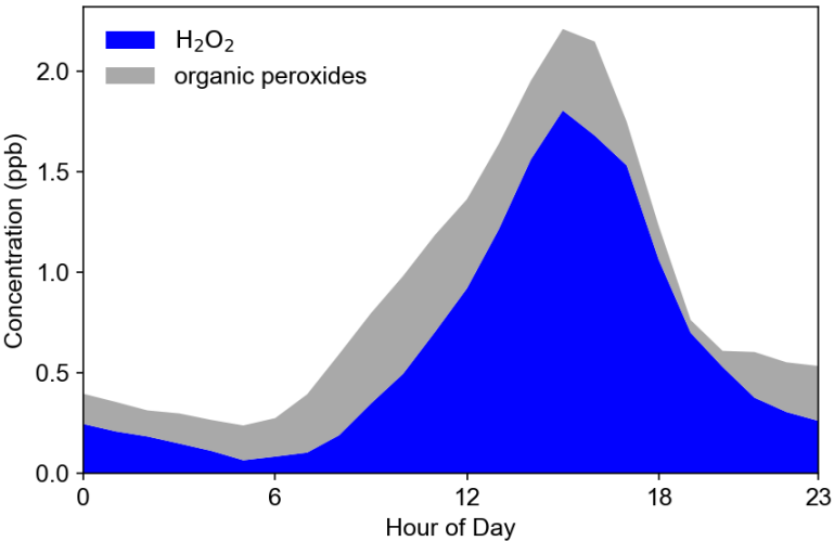
Figure 3. Average diurnal cycles of H 2 O 2 and organic peroxides (ROOH) observed throughout the entire campaign period at the SRE-RCEES site The concentrations of H 2 O 2 and organic peroxides.
