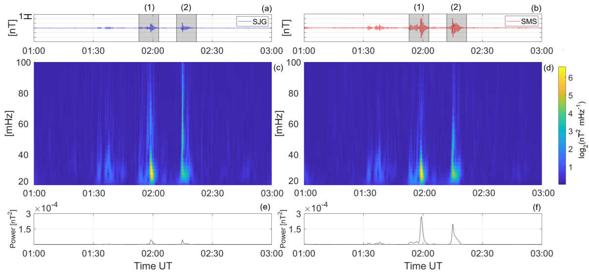
Figure 5. Pc3 pulsations (a-b), squared-wavelet coefficients scalograms (c-d) and global wavelet spectral (e-f). America-SAMA region.
