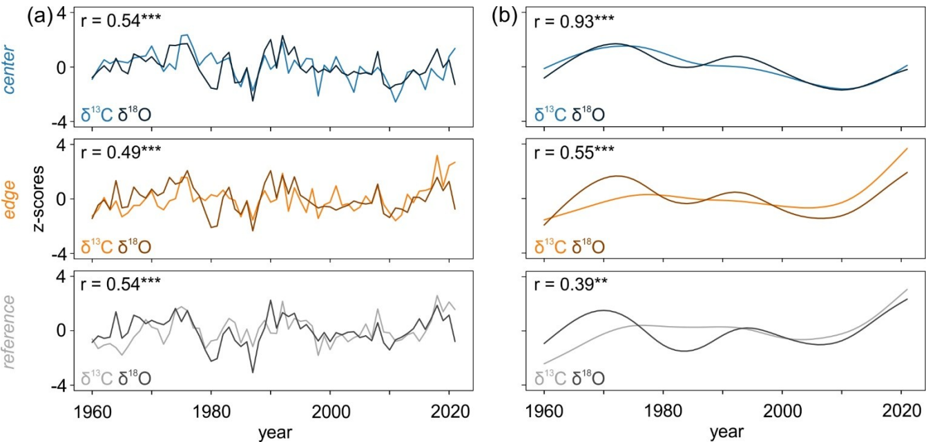
315 Figure 5. The relationship between \delta^{13}\text{C} and \delta^{18}\text{O} (a) raw chronologies and (b) 30-year low pass filters of raw chronologies ( ^{***} p < 0.001 , ^{**} p < 0.01 ).
