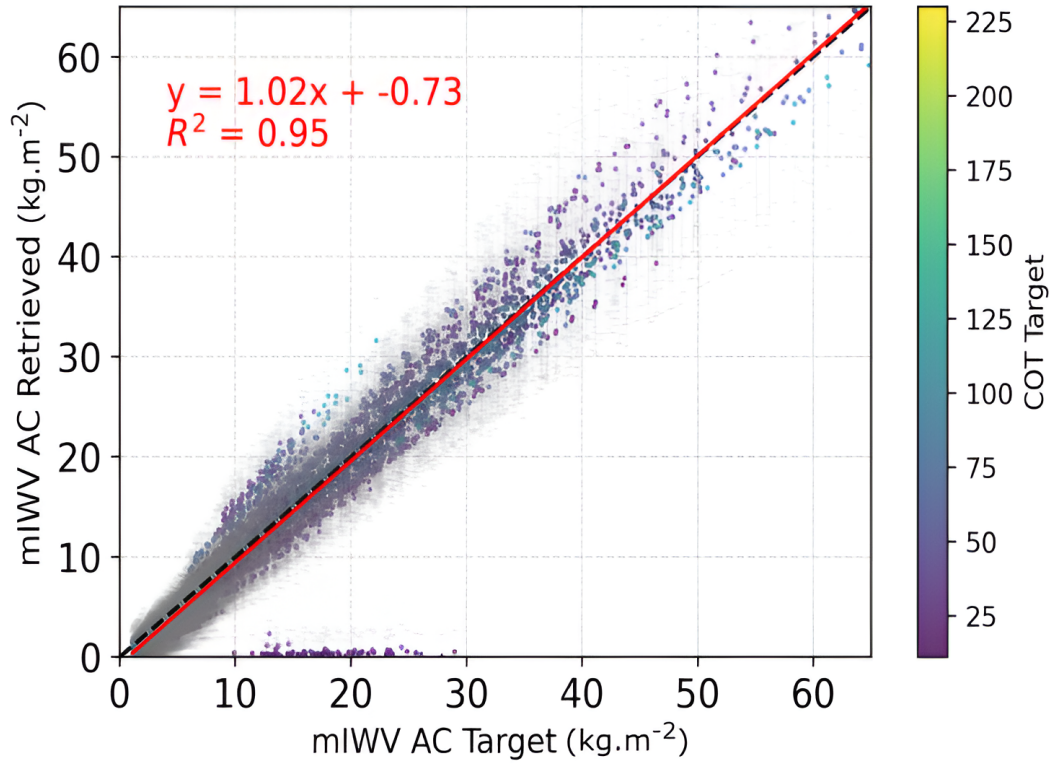
Figure 8. Relationship between the retrieved and target mIWV_{AC} values for profiles containing low-/mid-level clouds. The red line represents the linear regression and the black dashed line indicates the y = x line. Error bars represent the uncertainty estimated by the retrieval algorithm.
