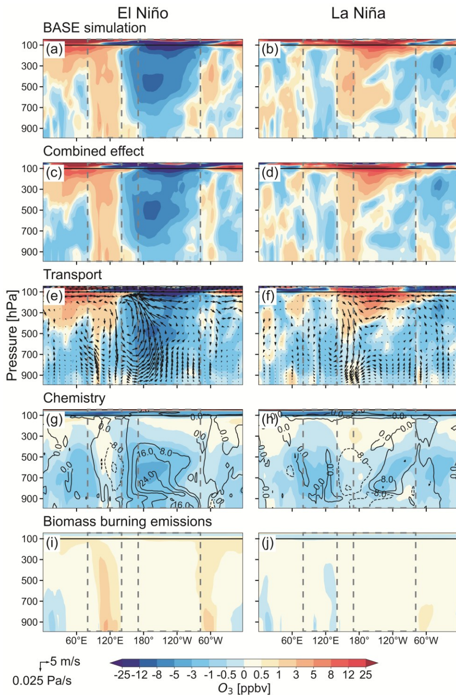
Figure 5. Similar to Figure 4, but showing the vertical distribution of ozone concentration in the equatorial region (5°S-5°N). Panels e-f overlay the difference in wind fields between the El Niño (La Niña) periods and the Normal periods. Panels g-h overlays the difference in
