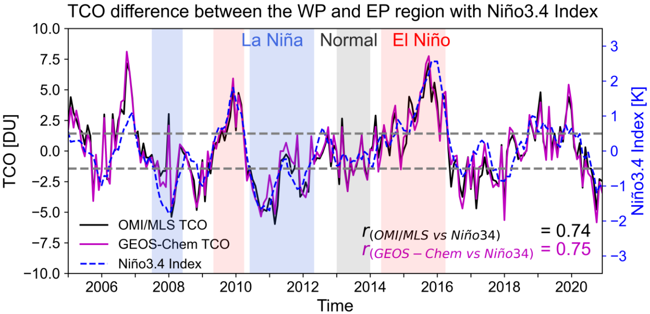
305 Figure 3. The difference in the deseasonalised and detrended TCO between WP and EP region over 2005-2020 from OMI (black lines) and GEOS-Chem simulation (purple lines). The Niño3.4 Index (blue dash lines) is also shown. The grey, red and blue shading in the figure represent the Normal (year 2013), El Niño, and La Niña periods, respectively. The El Niño and La Niña periods are defined as consecutive 1-2 years with the Niño3.4 index greater than 0.5 and less than -0.5 (Yeh et al., 2022), selected for sensitivity experiments in this study, respectively.
