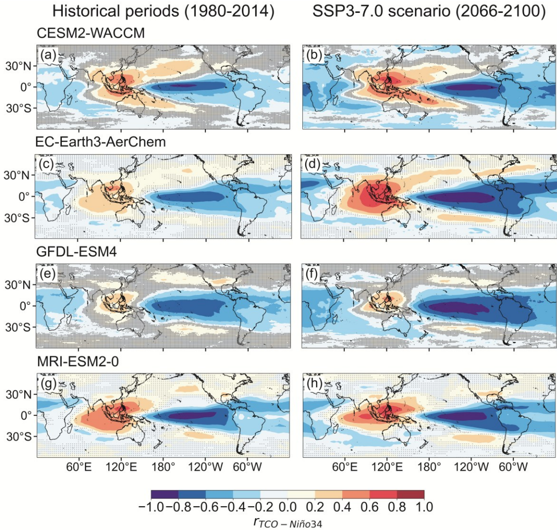
560 Figure 9. The r_{\text{TCO-Niño34}} in (a) historical (1980-2014) and (b) future (2066-2100) periods under the SSP3-7.0 scenario from four CMIP6 models with available future projections. Dots denote regions showing r_{\text{TCO-Niño34}} with p-values>0.05.
