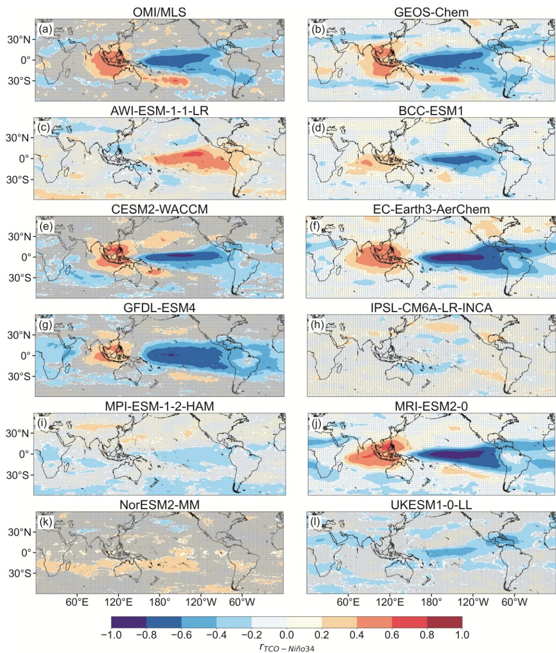
Figure 6. The r_{TCO-Ni\tilde{n}o34} over 2005-2014 from OMI/MLS satellite observations, GEOS-Chem and ten CMIP6 models results. Dots denote regions showing r_{TCO-Ni\tilde{n}o34} with p-values>0.05
