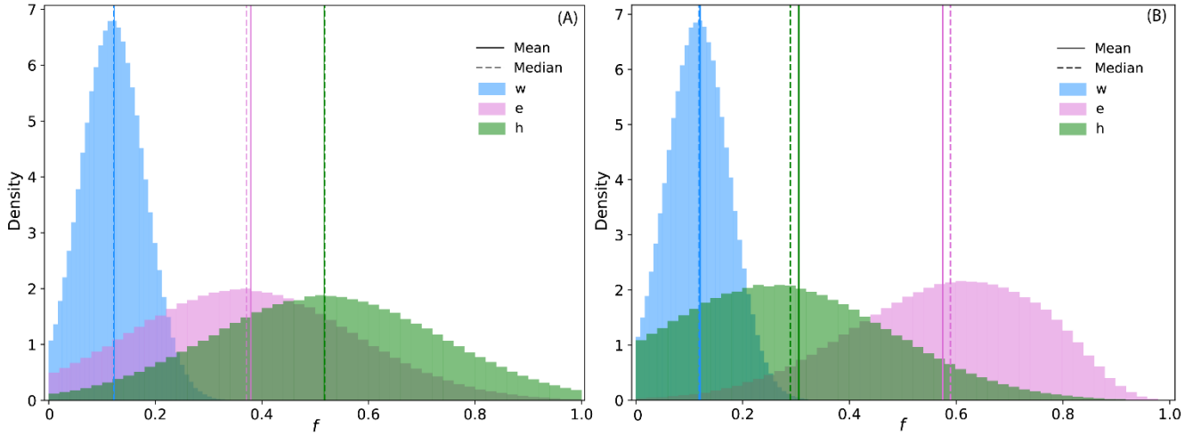
565 Figure 6. Distribution of the fraction of Si export as w_{river}^{Si} , e_{river}^{Si} , and h_{river}^{Si} , calculated using riverine Si concentrations, suspended sediments and the mass balance. The solid line represents the mean, while the dashed line indicates the median. (A) Results based on the mean estimated e_{river}^{Si} = 0.36 \pm 0.21 derived from turbidity-based suspended sediment estimates. (B) Sensitivity analysis assuming e_{river}^{Si} = 0.62 \pm 0.21 , corresponding to the quartz fraction of the bedrock, under the assumption that quartz is inert.
