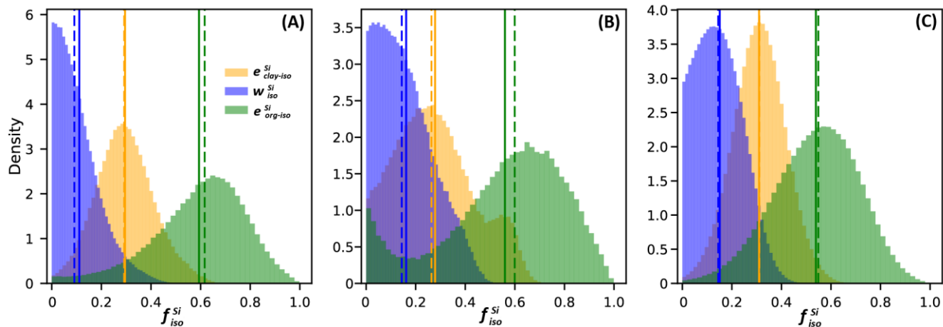
Figure 4. Distribution of the fraction of Si export as e_{clay-iso}^{Si} , e_{org-iso}^{Si} , and w_{iso}^{Si} calculated using the combined \delta^{30}\text{Si} and Ge/Si isotopic mass balance for three scenarios with varying signatures in the organic fraction. Solid lines represent the mean of each fraction, while dashed lines indicate the median. (A) Scenario 1 uses a uniform distribution for the plant signatures, incorporating all measured leaf values. (B) Scenario 2 uses a normal distribution using only the wheat signatures. (C) Scenario 3 uses a normal distribution using only the maize signatures.
