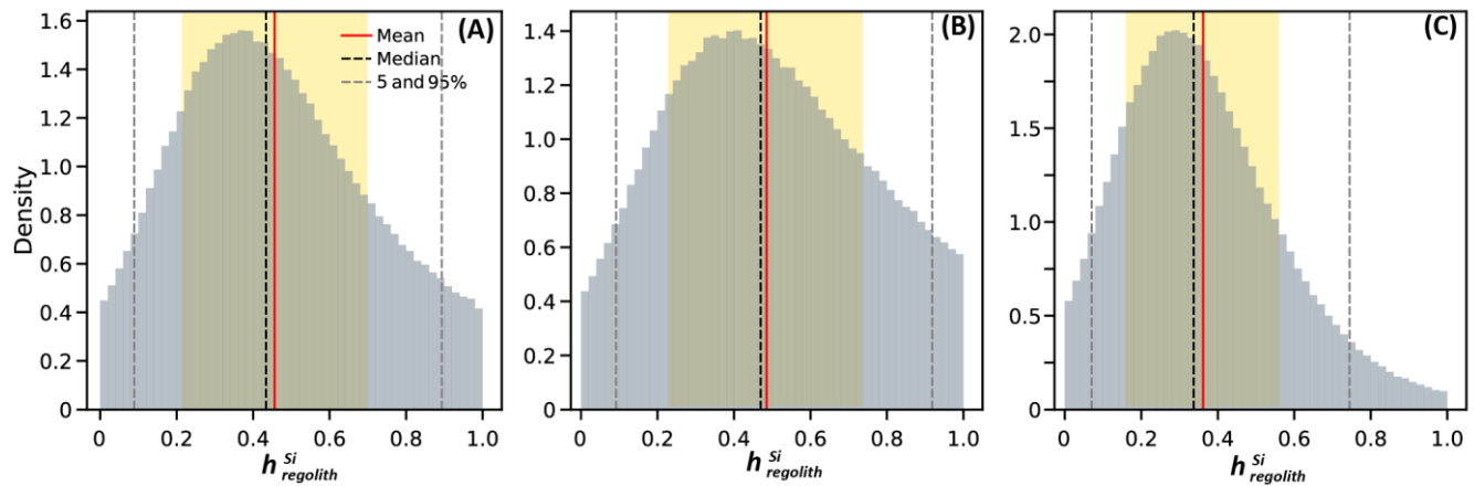
Figure 7. Distribution of the fraction of harvested Si ( h_{regolith}^{Si} ) calculated using Si loss indexes and isotopic fractionation for three scenarios with varying plant isotopic fractionation. Red lines indicate the mean, black dashed lines represent the median, and grey dashed lines mark the 5th and 95th percentiles. Yellow shaded areas denote the mean \pm one standard deviation (1 SD). (A) Scenario 1 uses a uniform distribution for the plants isotopic fractionation, incorporating all isotopic fractionations determined in leaves. (B) Scenario 2 uses a normal distribution based only on wheat isotopic fractionation. (C) Scenario 3 uses a normal distribution based only on the maize isotopic fractionation.
