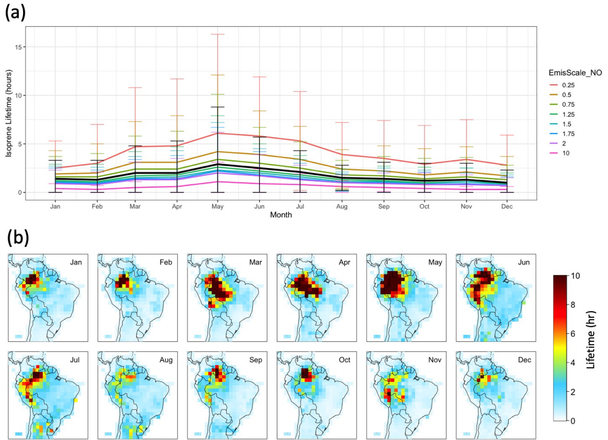
Figure 2: (a) Simulated monthly mean midday isoprene lifetime (hr) over Tropical South America with different NO x emission levels. Error bars indicate standard deviation over the studied region. (b) Monthly distribution of mean isoprene lifetime (hr) with default NO x emissions ( EmisScale_NO = 1).
