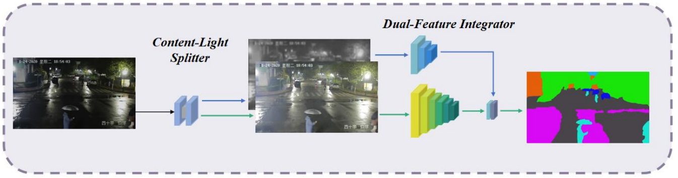
Figure 1: NWseg model inference process
