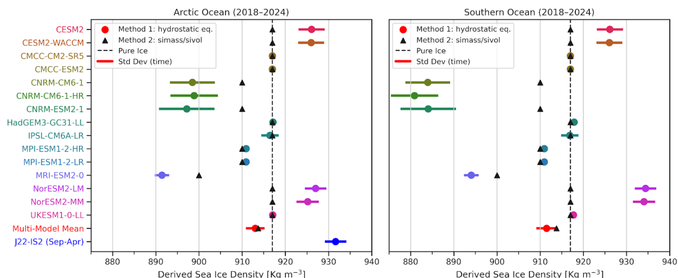
Figure 4: Derived bulk sea ice density in the 15 model CMIP6 subset (models with available freeboard, snow, and ice thickness data, not including ACCESS-CM2). Circles indicate the annual mean for each model and horizontal lines show the standard deviation across months (a proxy for the seasonality). A 50% SIC masking is applied before spatial averaging. The dashed vertical black line shows the 916 kg m -3 ‘pure ice’ bulk ice density assumption used in the IS2SITMOGR4 dataset. Also shown is the J22 ice density from IS2SITMOGR4 averaged between September and April 2018 to 2024.
