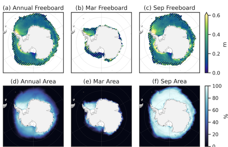
Figure 3: As in Figure 2 but for the Southern Ocean total freeboard (top) and sea ice concentration (bottom).
