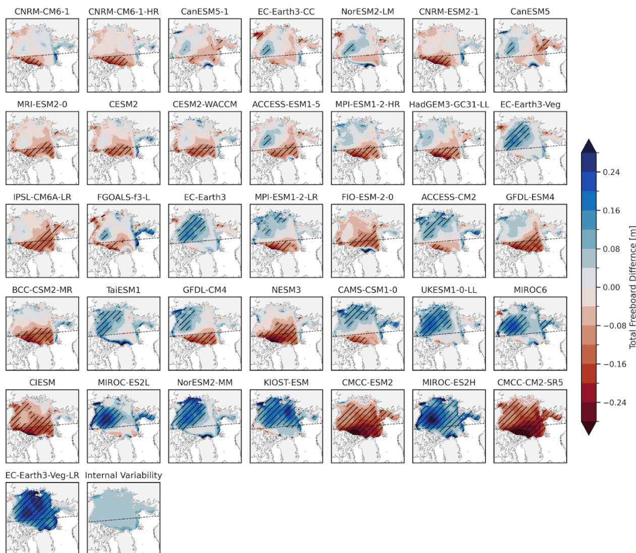
Figure 11: Total freeboard difference of the 2018 to 2024 annual mean for each CMIP6 model (ensemble mean) relative to ATL20 v4 (processed as discussed in Sect. 2 and 3). Models are shown in order of lowest (top left by row) to highest mean absolute error (MAE). The dashed line (50°E and 130°W meridians) is used for the Eastern and Western sector analysis. Note that only model grid cells within our Inner Arctic Ocean domain and which are ‘perennially ice-covered’ in ATL20 v4 are included here. Final panel shows our estimate of CMIP6 mean regional internal variability (two standard deviations, Sect. 2.3.3.)
