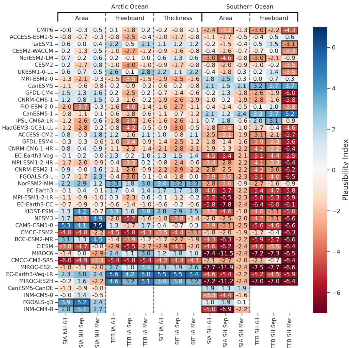
Figure 9: Plausibility assessment of the full 40 model CMIP6 suite for the individual model ensemble means and the multi-model CMIP6 mean, (top row) across all metrics, time-periods and hemispheres. The plausibility index ( \phi ) is calculated as in Eq. 7 using the 2015-2029 internal variability estimates and observational uncertainties listed in Table 2 (low uncertainty for the Arctic, high for the Southern Ocean). Models are sorted by the average \phi across all values shown, with the four models missing freeboard/thickness output included at the bottom and the CMIP6 mean included at the top. Values of \phi greater than 3 are outlined in black.
