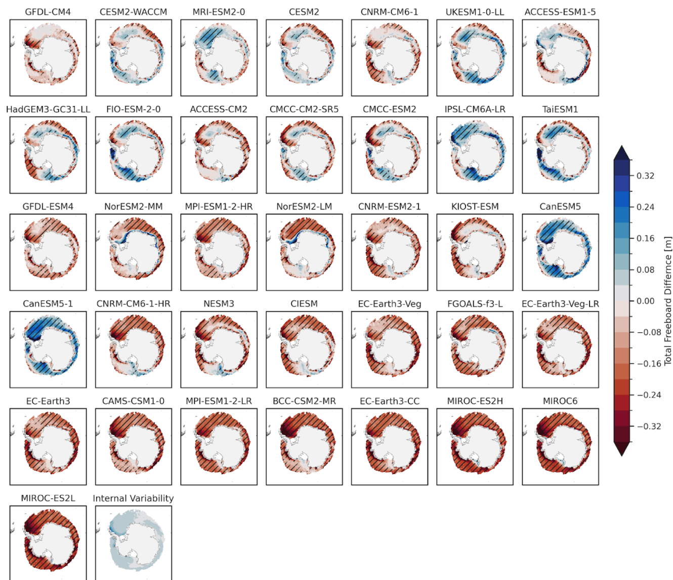
Figure 13: As in Figure 11 but for the Southern Ocean.
