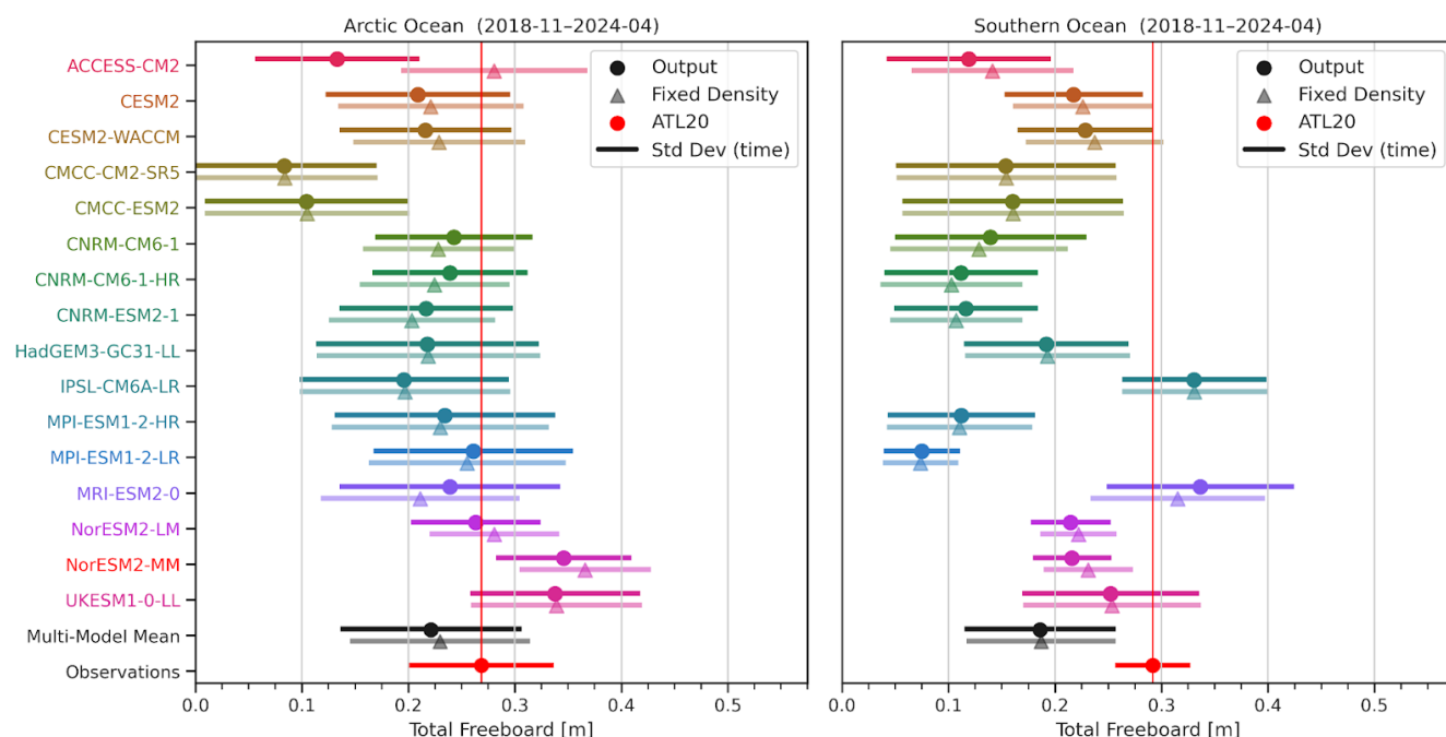
Figure 5: Comparison of mean Arctic Ocean (left) and Southern Ocean (right) total freeboard in the 16-model CMIP6 freeboard subset from the ensemble mean total freeboard output (circles), derived total freeboard assuming a fixed density of 916 Kg m -3 (triangles), and total freeboard observations from ATL20 v4 (processed as discussed in Sect. 2 and 3) (red) for the IS-2 study period (2018-11 to 2024-04). Horizontal lines show the seasonal variability (monthly standard deviation).
