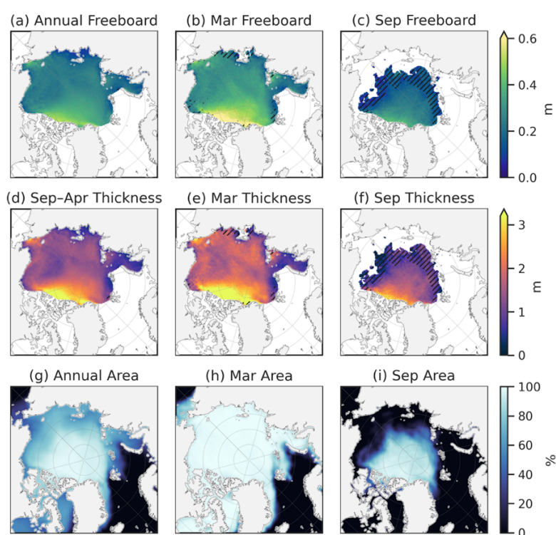
Figure 2: Total freeboard from ICESat-2 ATL20 v4 (top), sea ice thickness from ICESat-2 IS2SITMOGR4 v3 (middle), and sea ice concentration from OSI SAF (bottom) for Annual, March and September means in the 2018 to 2024 ICESat-2 period. The sea ice thickness annual mean only includes data between September and April due to data availability. The hatchings in the top two rows indicate grid-cells not included in the ‘perennial ice’ mask as data is missing from at least one year in the 2018 to 2024 period. Freeboard and thickness data are the interpolated/smoothed variables.
