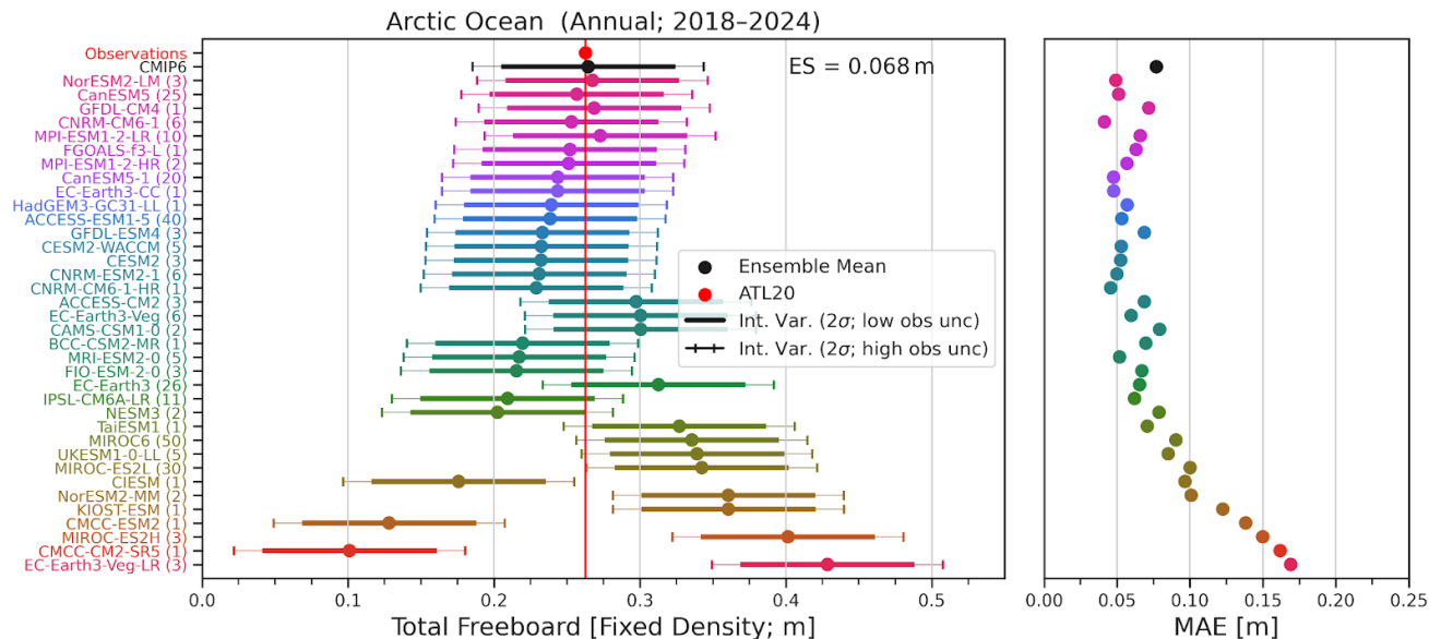
515 Figure 7: Comparisons of annual mean (2018 to 2024) Arctic Ocean total freeboard estimates from the 36-model CMIP6 subset (ensemble means, using a fixed ice density) and observations from ICESat-2 ATL20 v4 (processed as discussed in Sect. 2 and 3). Horizontal lines on each model show the plausibility window based on internal variability and both the low (bars) and high (whiskers) observational uncertainty estimates. The red circle and vertical red line shows the ATL20 observational mean. ES: ensemble spread. Right panel shows the Mean Absolute Error (MAE) of the spatial differences across the 25 km x 25 km grid-cells.
