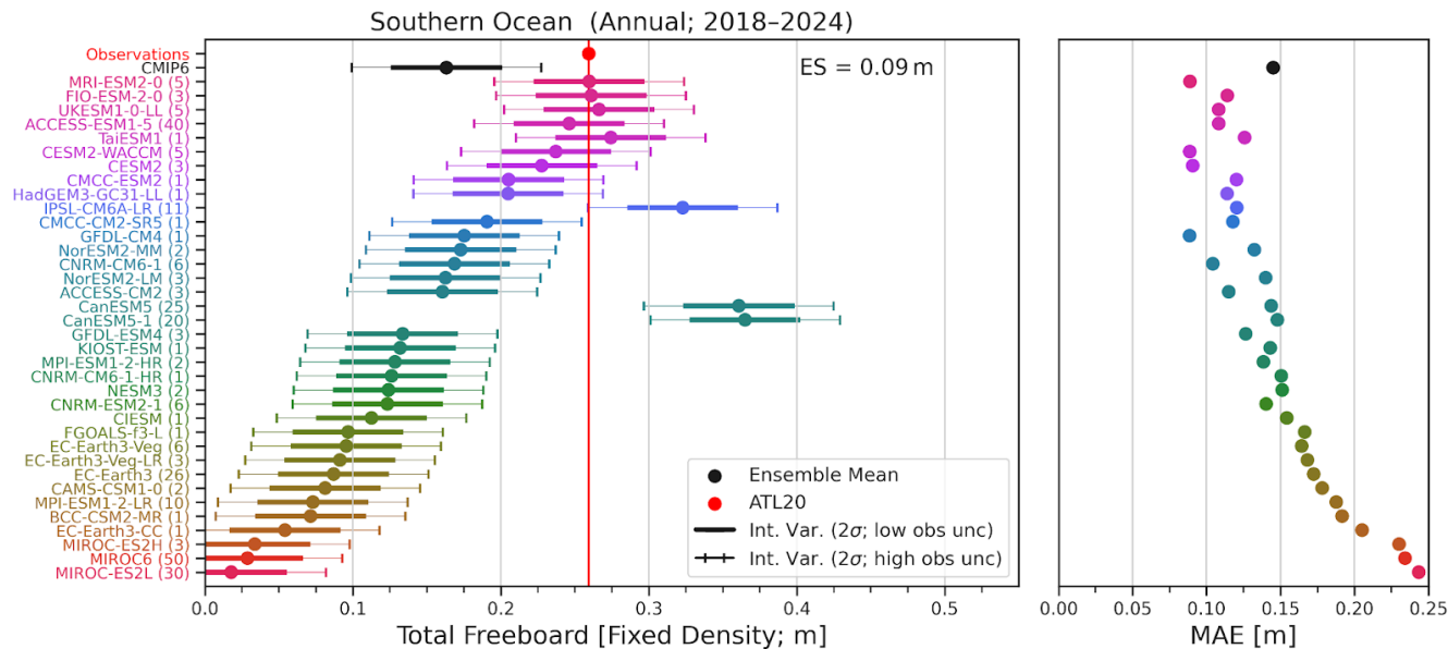
520 Figure 8: As in Fig. 7, but for the Southern Ocean.
