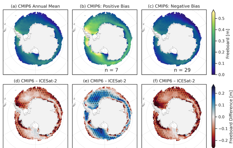
Figure 14: As in Figure 11, but for the Southern Ocean freeboard. No regional bias composite is shown—only composites where basin-averaged differences from ATL20 v4 are either positive or negative.
