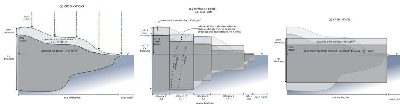
Figure 1: Schematic showing (a) observations of sea ice total freeboard from laser altimetry towards estimates of sea ice thickness, (b) advanced physics and ice thickness distribution typical of state-of-the-art sea ice models, (c) fixed ice thickness/snow parameterization used in more basic sea ice models. Note that ice freeboard is the extension of sea ice above sea level, while total freeboard is the extension of the ice and snow layer above freeboard. Sea ice models do not typically simulate freeboard, but this can be estimated based on an assumption of isostasy.
