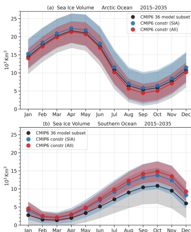
Figure 10: Seasonal CMIP6 ensemble mean sea ice volume (lines and circles) and ensemble spread (shading, one standard deviation) from the unconstrained 36-model subset (black), the annual area constrained subset (blue), and the subset constrained with all considered annual variables, including area and freeboard for both hemispheres, and the addition of sea ice thickness for the Arctic only (red).
