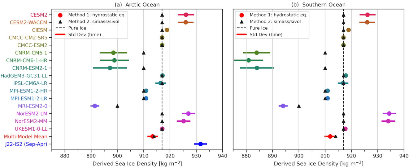
Figure 4: Derived mean (a) Arctic Ocean and (b) Southern Ocean bulk sea ice density in the 16 model CMIP6 subset (models with available freeboard, snow, and ice thickness data, not including ACCESS-CM2). Circles indicate the annual mean for each model and horizontal lines show the standard deviation across months (a proxy for the seasonality). A 50% SIC masking is applied before spatial averaging. The dashed vertical black line shows the 916 kg m -3 ‘pure ice’ bulk ice density assumption used in the IS2SITMOGR4 dataset. Also shown is the J22 ice density from IS2SITMOGR4 averaged between September and April 2018 to 2024.
