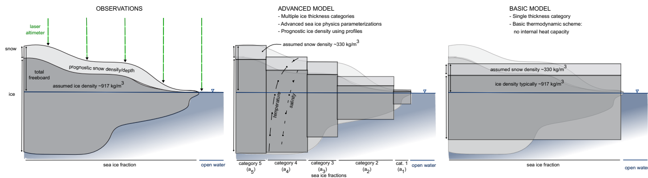
Figure 1: Schematic showing (left) observations of sea ice total freeboard from laser altimetry towards estimates of sea ice thickness, (middle) advanced physics and ice thickness distribution typical of state-of-the-art sea ice models, (right) fixed ice thickness/snow parameterization used in more basic sea ice models. Note that ice freeboard is the extension of sea ice above sea level, while total freeboard is the extension of the ice and snow layer above freeboard. Sea ice models do not typically simulate freeboard, but this can be estimated based on an assumption of isostasy.
