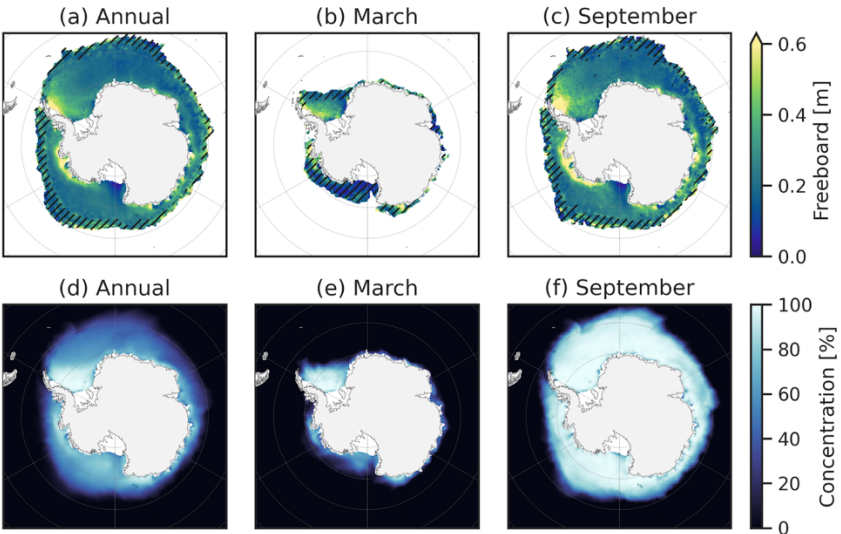
280 Figure 3: As in Fig. 2 but for the (a, b, c) Southern Ocean total freeboard and (d, e, f) sea ice concentration.
