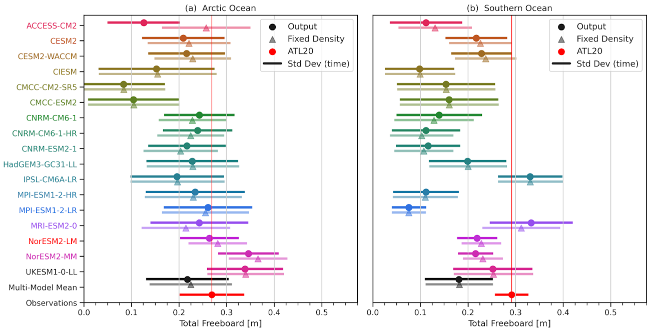
Figure 5: Comparison of the mean (a) Arctic Ocean (b) and Southern Ocean total freeboard in the 17-model CMIP6 freeboard subset from the ensemble mean total freeboard output (circles), derived total freeboard assuming a fixed density of 916 kg m -3 (triangles), and total freeboard observations from ATL20 v4 (processed as discussed in Sect. 2 and 3) (red) for the ICESat-2 study period (2018-11 to 2024-04). Horizontal lines show the seasonal variability (monthly standard deviation).
