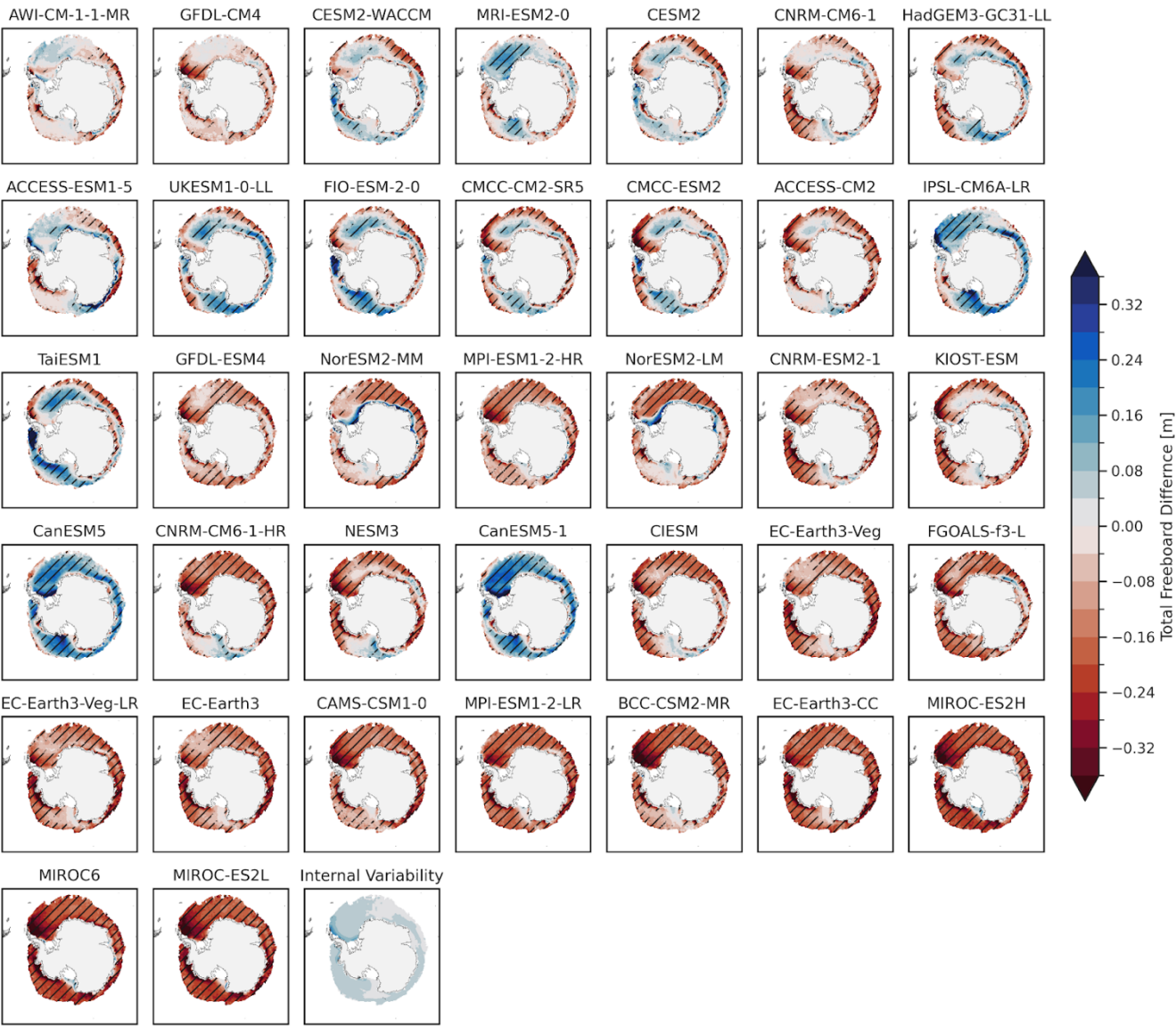
Figure 13: As in Fig. 11 but for the Southern Ocean.
