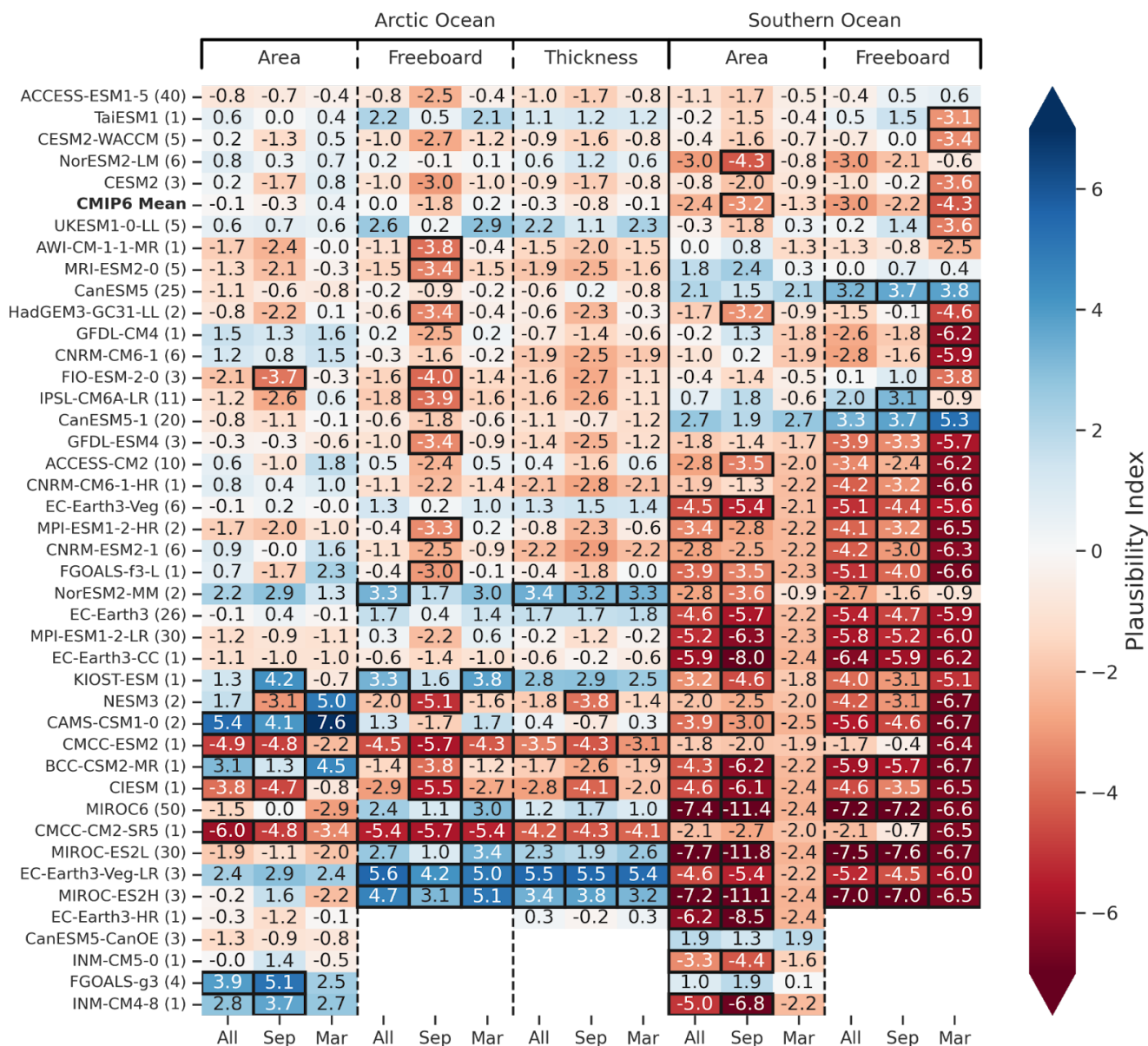
Figure 9: Plausibility assessment of the full 40 model CMIP6 suite for the individual model ensemble means and the multi-model CMIP6 mean, (top row) across all metrics, time-periods and hemispheres. The plausibility index ( \phi ) is calculated as in Eq. 7 using the 2015-2029 internal variability estimates and observational uncertainties listed in Table 3 (low uncertainty for the Arctic, high for the Southern Ocean). Models are sorted by the average \phi across all values shown, with the four models missing freeboard/thickness output included at the bottom and the CMIP6 mean included at the top. Lower values are considered more plausible. Values of \phi greater than 3 are outlined in black.
