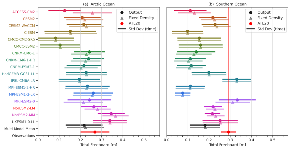
Figure 5: Comparison of the mean (a) Arctic Ocean and Southern Ocean total freeboard in the 17 model CMIP6 freeboard subset from the ensemble mean total freeboard output (circles), derived total freeboard assuming a fixed density of 916 kg m -3 (triangles), and total freeboard observations from ATL20 v4 (processed as discussed in Sect. 2 and 3) (red) for the ICESat-2 study period (2018-11 to 2024-04). Horizontal lines show the seasonal variability (monthly standard deviation).
