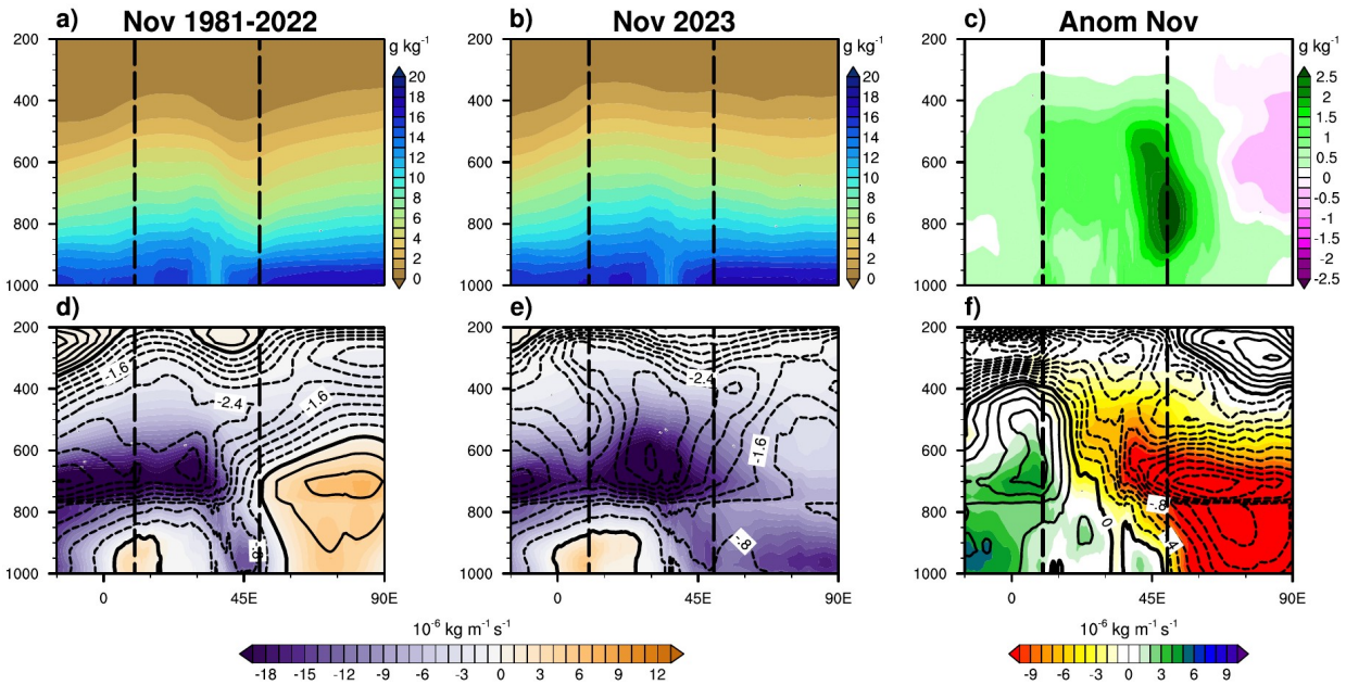
398 Fig 5: Longitude-height cross-sections of (first row) specific humidity and (second row) zonal 399 moisture flux (shaded: 10^{-6} \text{ kg m}^{-1} \text{ s}^{-1} ) and zonal wind (contour: \text{m s}^{-1} ) for (a,d) the climatology of 400 November 1981-2022, (b,e) November 2023 and (c,f) the anomaly, averaged between 10° S-10° N. 401 The dashed black lines denote the limits of EA.
