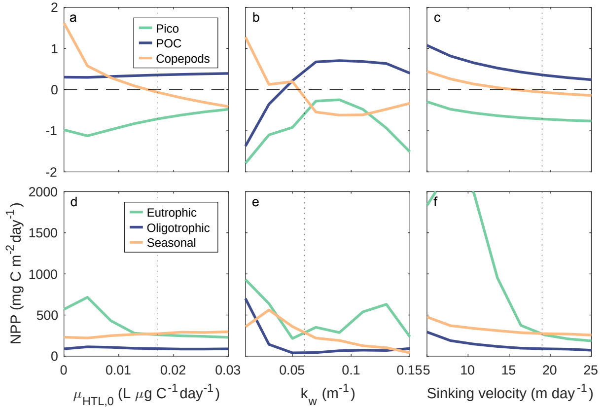
Figure E5. Sensitivity analysis of the parameters: higher trophic level mortality \mu_{\text{HTL},0} , light extinction coefficient k_w , and sinking velocity u . Top row: the objective function for comparison with pico-plankton, POC, and copepods (see Fig. 6. Bottom row: NPP at three characteristic water columns extracted from global simulations.
