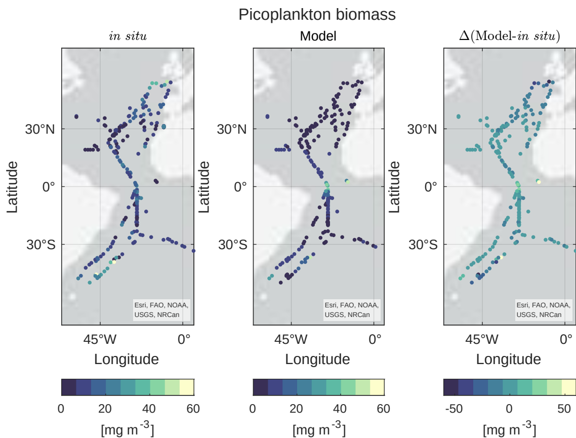
Figure D4. Comparison of picophytoplankton in situ data (Martínez-Vicente et al., 2017) with model picoplankton biomass. Basemap: Esri, FAO, NOAA, USGS, NRCan; powered by Esri.
