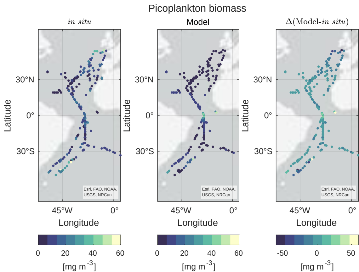
Figure D4. Comparison of picophytoplankton in situ data with model picoplankton biomass.
