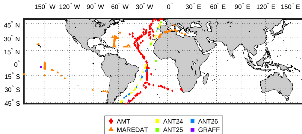
Figure D3. Picophytoplankton Cruises transects
