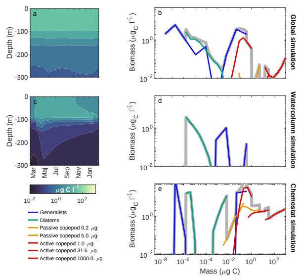
Figure E2. Same as in fig. E1, but at an oligotrophic location (24°N, 158°W).
