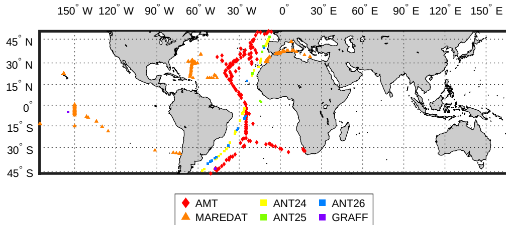
Figure D3. Picophytoplankton Cruises transects transects from Martínez-Vicente et al. (2017) .
