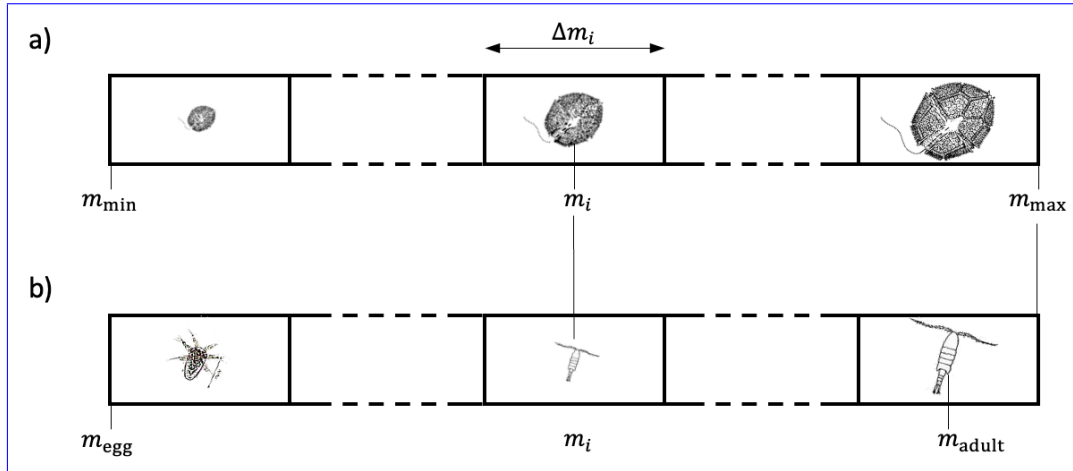
Figure A1. Specification of the computational grid used for unicellular organisms (a) and multicellular organisms (b). The grid for each unicellular plankton group (generalists and diatoms) contain n contiguous size groups in the range from m_{\min} and m_{\max} . Each size group is defined by its central mass (geometric mean) m_i . For multicellular plankton the grid for each group is from m_{\text{egg}} . The last size group has the central mass m_{\text{adult}} . This means that copepods actually becomes adult at smaller mass than m_{\text{adult}} , and that the last size group spans a range of masses.
