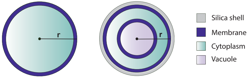
Figure 2. Geometry of generalist and diatom cells
