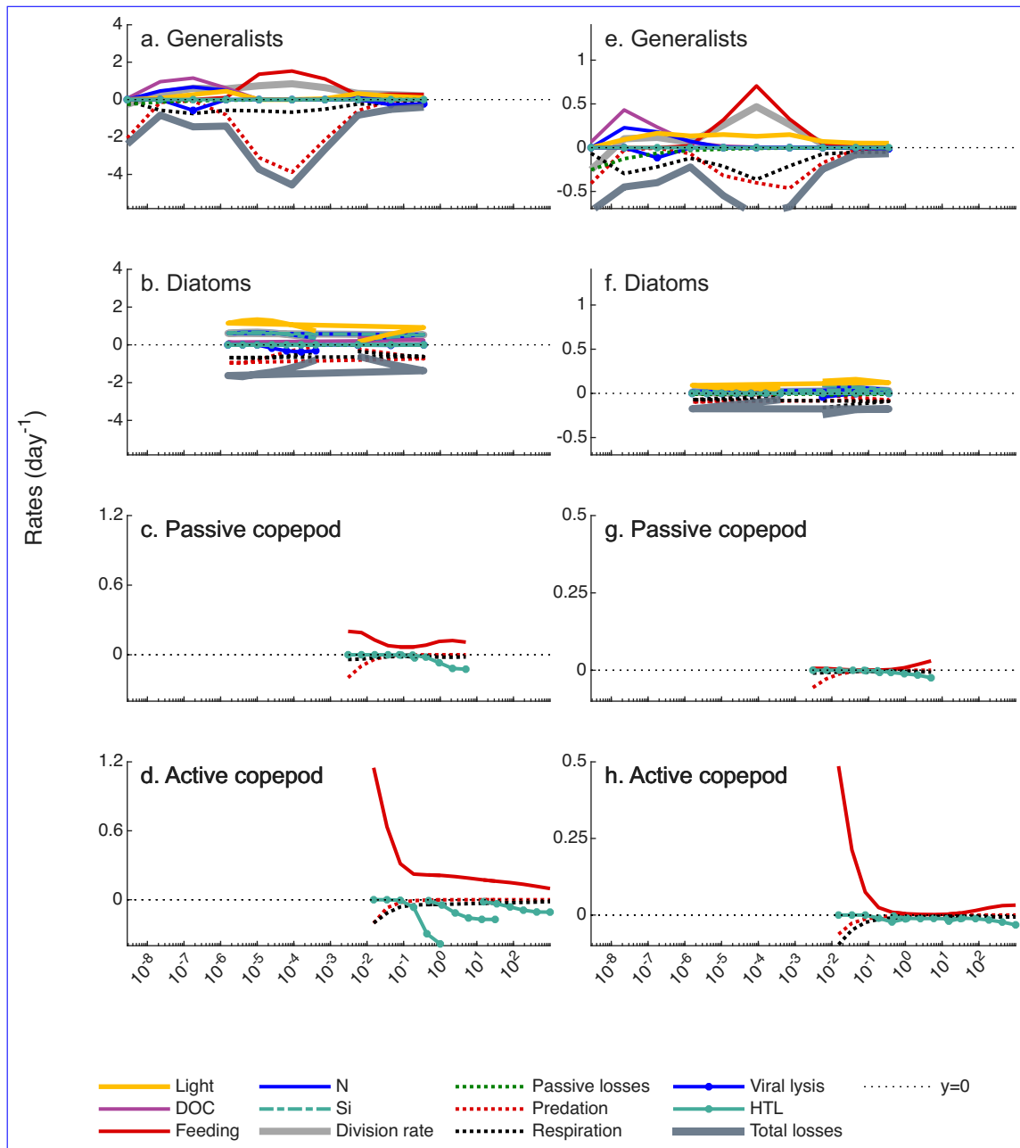
Figure 16. Gains and losses as a function of cell/body size in the spring bloom (April, left) and the summer (July, right) from the chemostat simulation in Fig. 15e . The lines above the horizontal dashed line shows gains either of carbon (from DOC uptake or photoharvesting; magenta and yellow), nutrients, silicate (blue and green), or a combination of carbon and nutrients from predation (red). The lines below the dashed lines shows losses of carbon from respiration (dashed black) or mortalities from predation (dashed red) or viral lysis (blue). The division rate is shown with thick grey. The output is from the chemostat simulation in Fig. 15d. Note the differences in the y-axes ranges between the left and right columns.
