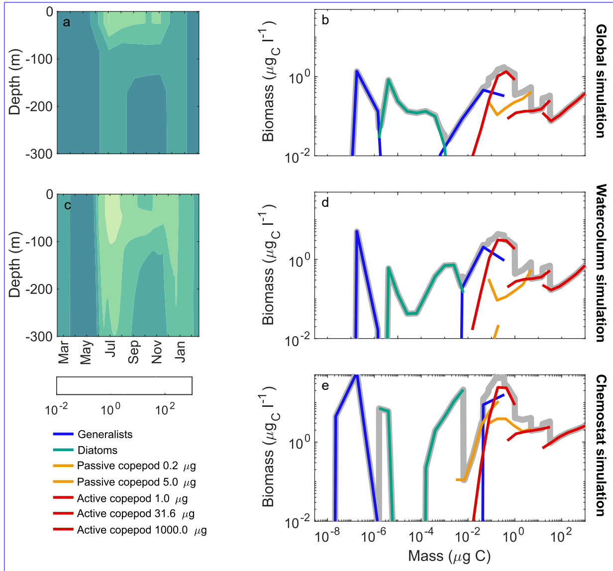
Figure 15. Model output for a 10-year simulation in the global, water column, and chemostat environments at a seasonally stratified location ( 60^\circ\text{N} , 40^\circ\text{W} ) (red star in Fig. 7). (a) Total biomass in a water column extracted from the global simulation. (c) Total biomass in the same water column, but extracted from the water-column simulation. (b),(d),(e): Sheldon spectrum of the community from global, water-column, and chemostat simulations at 5 meters depth and geometrically averaged over the last year. See Fig. 5 for an indicative length axis.
