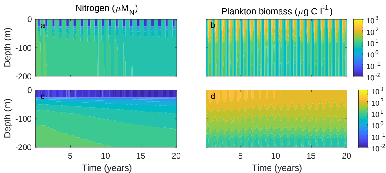
Figure E6. Convergence of a global simulation in a seasonal environment ( 60^\circ\text{N} , 40^\circ\text{W} ; a,b) and at equator ( 0^\circ\text{N} , 15^\circ\text{W} ; c,d).
