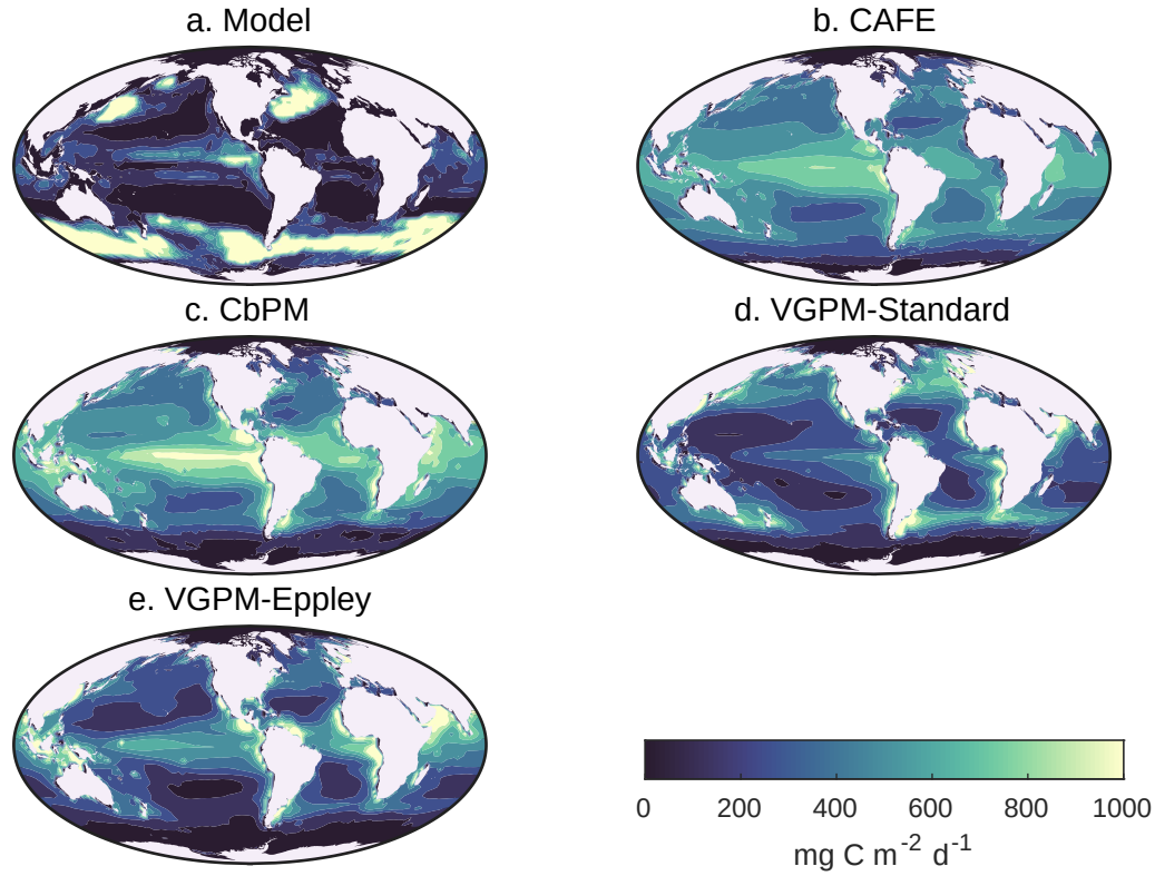
Figure 8. (a) NUM annual mean NPP, (b) CAFE estimated annual mean NPP (Silsbe et al., 2016), (c) CbPM estimated annual mean NPP (Westberry et al., 2008), (d) VGPM-Standard estimated annual mean NPP (Behrenfeld and Falkowski, 1997), and (e) VGPM-Eppley estimated annual mean NPP (Behrenfeld and Falkowski, 1997), all datasets from (Ocean Productivity). Units are \text{mg C m}^{-2} \text{ d}^{-1} .
