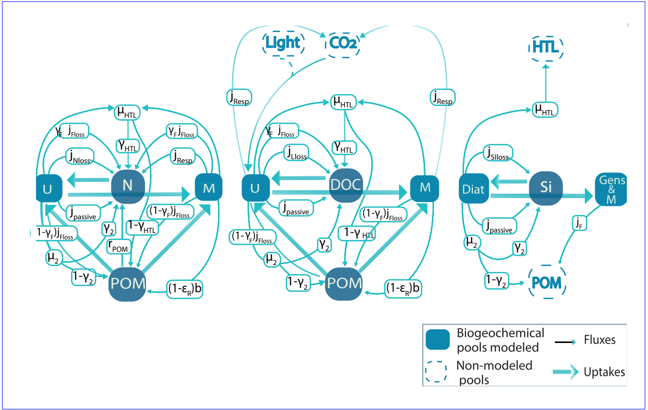
Figure 4. Representation of nitrogen, carbon and silica fluxes in unicellular (generalists and diatoms) (U) and multicellular (M) plankton. All rates are in units \text{day}^{-1} . In the chemostat setup POM sinks out to the deep (Eq. 20). The j 's represent direct losses, the \mu 's represent mortalities, \gamma 's represent fractioning of a flux into different pools (e.g. between direct remineralization and to POM), b = J_{\text{in},1}/m_{\text{egg}} is the copepod birth rate, and \varepsilon_F is feeding efficiency. \gamma_{\text{POM}} = 1 - \gamma_{\text{HTL}} , and j_{\text{Nloss}} refers to the losses of N and Si when growth is negative, and surplus carbon from photosynthesis to DOC. Note that POM does not contain silicate, instead all silicate fluxes that should have gone into POM are considered lost to the deep sea, therefore also absent in the model. Similarly, we assume that none of the silica in diatoms is assimilated by their predators and it is all instead directly remineralized.
