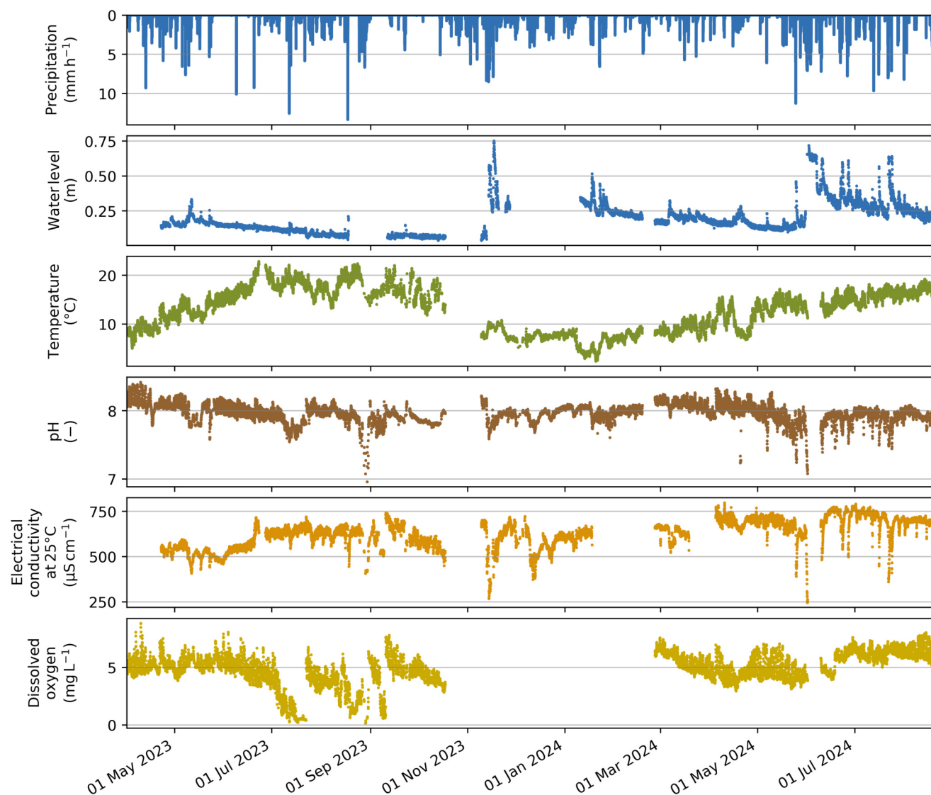
Figure 3. Continuous measured data on water level, temperature, pH value, electrical conductivity, and dissolved oxygen, complemented with precipitation data (DWD Climate Data Center (CDC), 2024), from Apr. 2023 to Aug. 2024.
