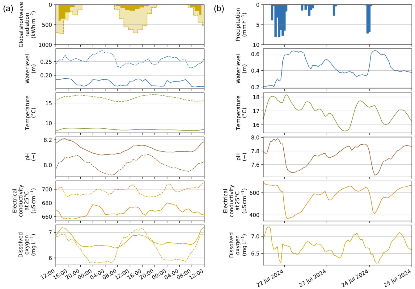
Figure 4. Zoom on continuous measured data on water level, temperature, pH value, electrical conductivity, and dissolved oxygen, complemented with precipitation and radiation data (DWD, 2024); (a): Zoom on 48 h to visualize daily fluctuations for typical summer (dashed: 3-5 Aug. 2024) and winter days (continuous: 27-29 Feb. 2024); (b): Zoom on flood event (3.5 days) in July 2024.
