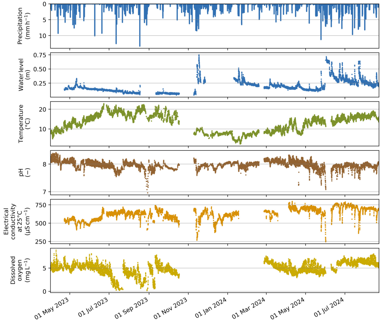
Figure 3. Continuous measured data on water level, temperature, pH value, electrical conductivity, and dissolved oxygen, complemented with precipitation data (DWD, 2024), from Apr. 2023 to Aug. 2024.
