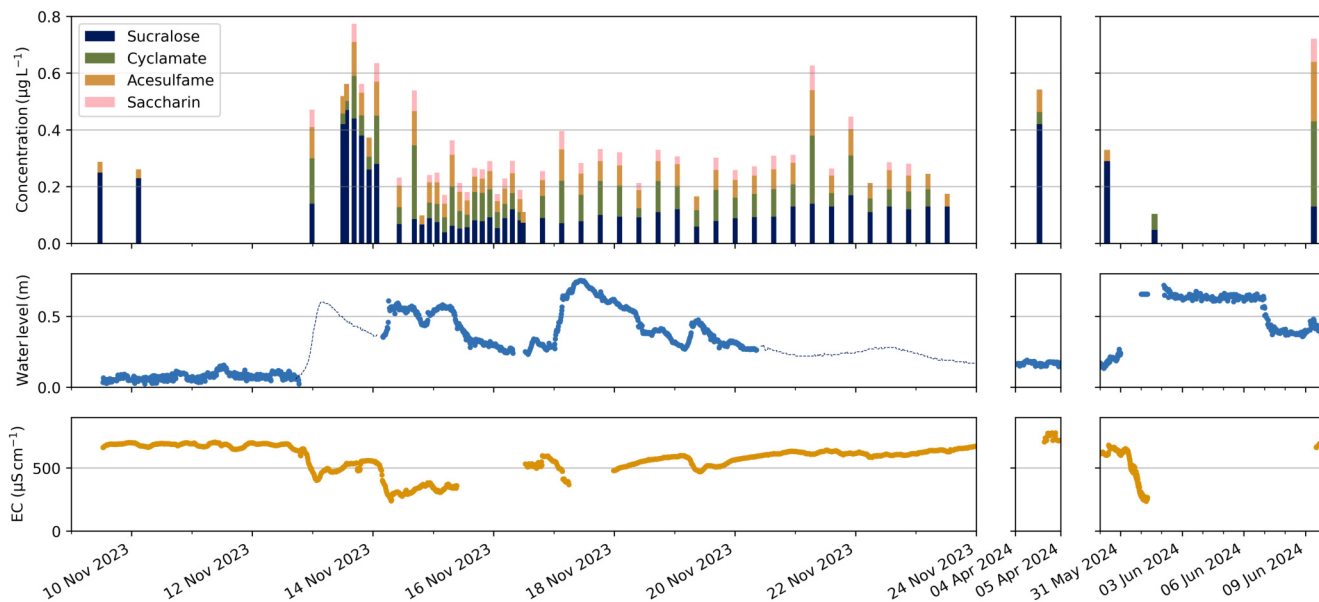
Figure 7. Concentrations of four artificial sweeteners (sucralose, cyclamate, acesulfame, saccharin) over three periods (Nov. 2023, Apr., and June 2024) plotted with the water level and EC measurements of the monitoring kit. In the periods in which no water level measurements were available from the monitoring kit, the timeline was supplemented with measurements from the Lauben gauge downstream (thin dashed line).
