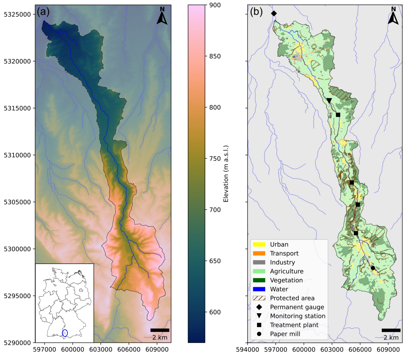
Figure 1. Study area map of (a) elevation in the catchment, which is the eastern tributary of the Günz River in Bavaria, Germany (Bavarian Surveying and Mapping Authority, 2022a) and (b) land cover (Bavarian Surveying and Mapping Authority, 2022b). The overview map in (a) displays the study area location in Germany.
