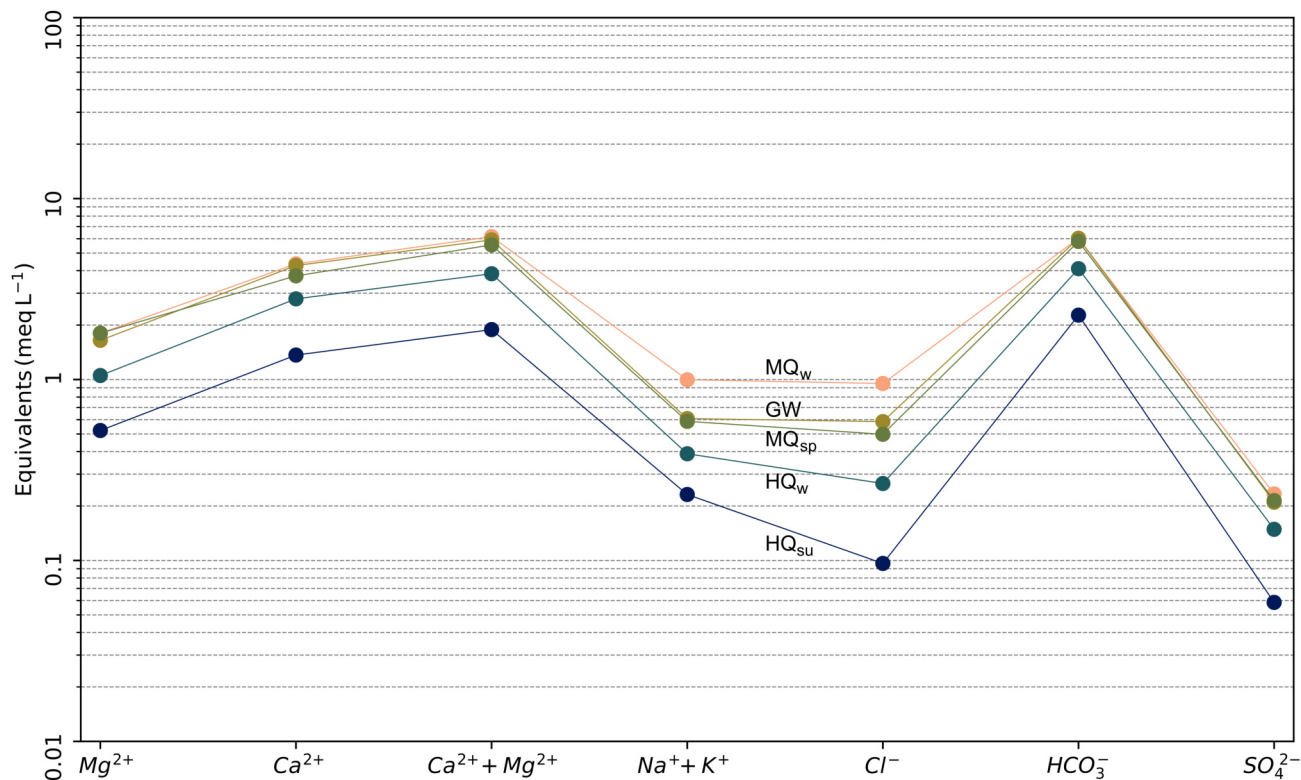
Figure 6. Schoeller plot with major ion concentrations for five water samples: mean discharge in winter (7 Dec. 2023, MQ w ), mean discharge in spring (4 Apr. 2024, MQ sp ), high discharge in winter (7 Nov. 2023, HQ w ), very high discharge in summer (1 June 2024, HQ su ), and groundwater in well 1 (4 Apr. 2024, GW).
