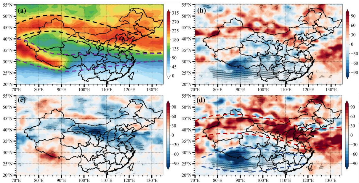
285 Figure 5: (a) The AMJ-averaged ozone STT flux ( \text{kg km}^{-2} \text{ month}^{-1} ) during 1980-2014. Composite anomalies of ozone STT flux ( \text{kg km}^{-2} \text{ month}^{-1} ) during (b) positive years, (c) negative years, and (d) their differences. Dashed lines denote the northern and southern branches of ozone STT flux, respectively. Black dots indicate the composite anomalies passing the 90 % confidence level based on the Student's t-test.
