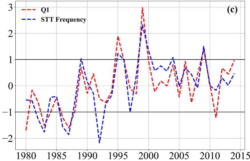
Figure 3: Heterogeneous correlations of (a) TP thermal forcing, where the black line represents the isoline of altitude at 3000 m outlining the area of the TP, (b) STT frequency, where the red and blue dashed lines denote the northern and southern branches of STT frequency, respectively, and (c) their normalized temporal coefficients in the first SVD mode (SVD1). Black dots mean passing the 90 % confidence level based on the Student's t-test.
