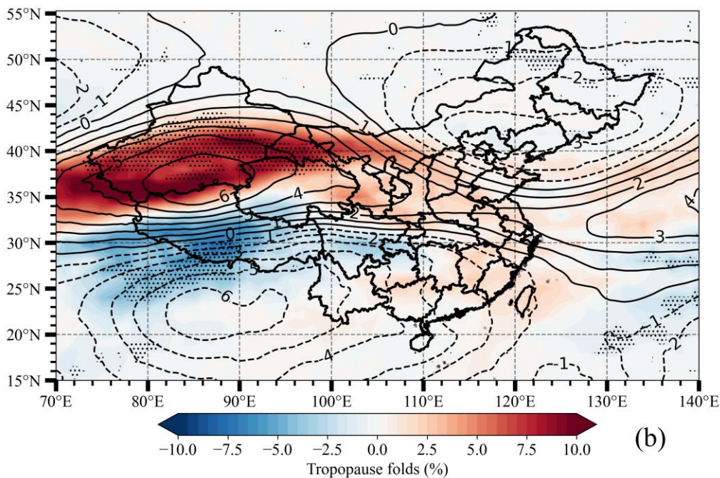
325 Figure 6: Composite differences in (a) geopotential height (shaded, gpm) and wind vectors at 200 hPa, (b) tropopause fold frequency (shaded, %) and zonal wind speed at 200 hPa (contour, m/s) with solid (dashed) contours representing an enhancement (attenuation) in westerly jet. Black dots and purple vectors indicate the composite anomalies passing the 90 % confidence level based on the Student's t-test.
