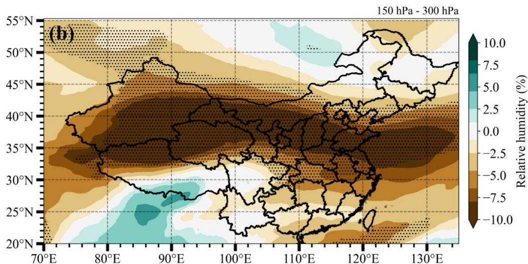
345 Figure 7: Composite differences in (a) potential vorticity (PVU) and (b) relative humidity (%) averaged in the UTLS from 150 hPa to 300 hPa between positive and negative Q1 anomaly years. Black dots indicate the composite anomalies passing the 90 % confidence level based on the Student's t-test.
