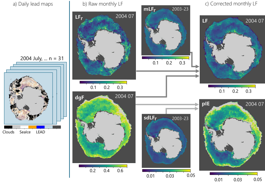
Figure 1. Retrieval of monthly lead frequency (LF) from daily lead maps: (a) Daily lead maps for July 2004 with categories cloud, sea ice, lead, artefact, (b) raw monthly lead frequency ( LF_r ) and data gap frequency (dgF) derived from daily data, and (c) corrected monthly lead frequency (LF) and the potential Integration Error (pIE) derived from the overall mean LF_r ( mLF_r ), the standard deviation of LF_r ( sdLF_r ), and monthly dgF.
