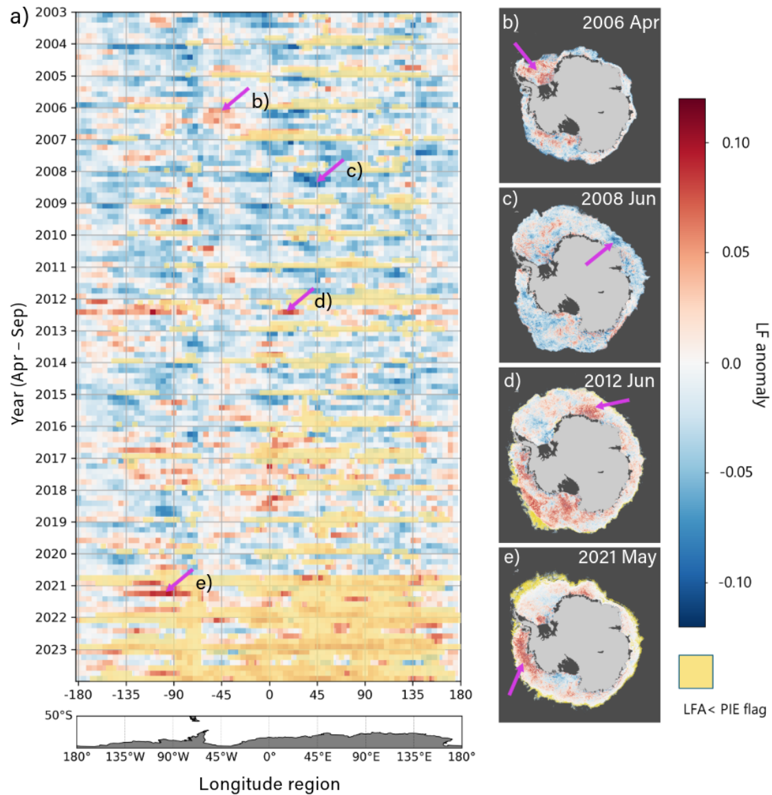
Figure 6. (a) Latitude-averaged ( 60^{\circ} to 90^{\circ} S) monthly lead frequency (LF) anomalies in 5^{\circ} longitude bins from April 2003 to September 2023. Areas that do not meet the LFA > pIE criterion are highlighted in yellow color. (b–e) Monthly LF anomaly maps of selected years and months from the left panel (a) are shown. Strong lead anomalies can be seen, for example, in (b) April 2006, (d) June 2012 and (e) May 2021. Anomalies are calculated relative to the climatological monthly mean.
