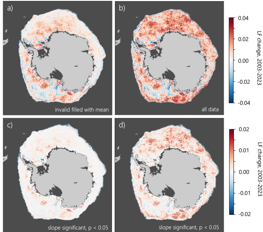
Figure 7. Lead frequency (LF) change from 2003 to 2023 according to linear trend in annual LF values for (a) where low-quality LF data (LFA < pIE) are replaced by the overall mean LF per pixel, (b) all LF data including low-quality LF, (c) and (d) only for where the slope of the linear trend in (a) and (b) , respectively, is significant at the 5 % level according to a two-tailed test.
