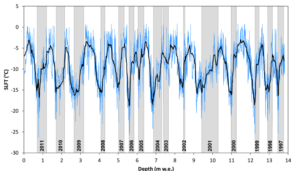
Figure 6: Snow layer formation temperature (SLFT) modelled at the drilling site by EISMModel from September 1, 1996 to September 30, 2011. The black line is a 100-order centred moving average. The grey bars represent months from October to January (when pollen is not released, Fig. 7), in order to facilitate the following comparisons. The year is referred to the month of January (e.g., winter 1996-‘97 is indicated as ‘1997’).
