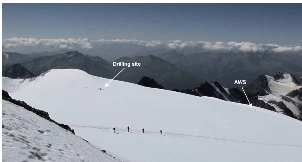
133 Figure 2: Photo of the upper accumulation area of Alto dell'Ortles Glacier taken from the summit of Mt. Ortles on 31 134 August 2015.
