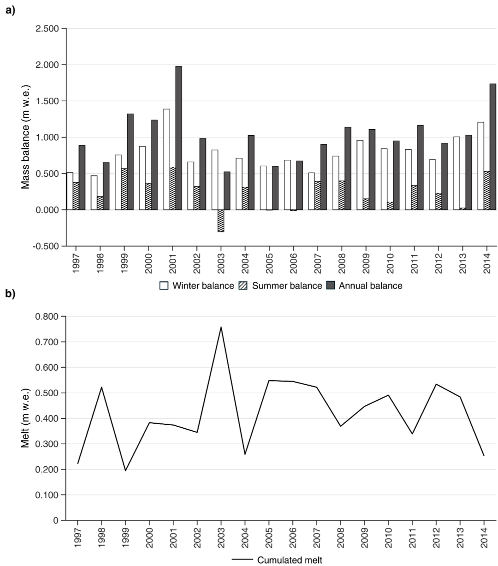
264 Figure 5: Interannual variability of a) seasonal and annual balance, and b) annual cumulated melt based on EISModel 265 calculation at the Ortles drilling site.
