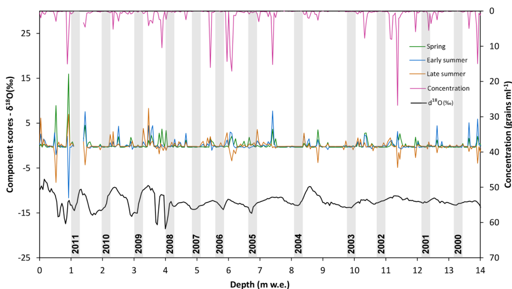
Figure 7: Concentration and principal component scores representative of spring, early summer and late summer of pollen data extracted from the Mt. Ortles core 1, compared with the \delta^{18}\text{O} values determined in the same core. Grey bars represent mid-winter months (December and January) based on pollen data, and have arbitrary width. Annual layer counting is based on \delta^{18}\text{O} and pollen evidence.
