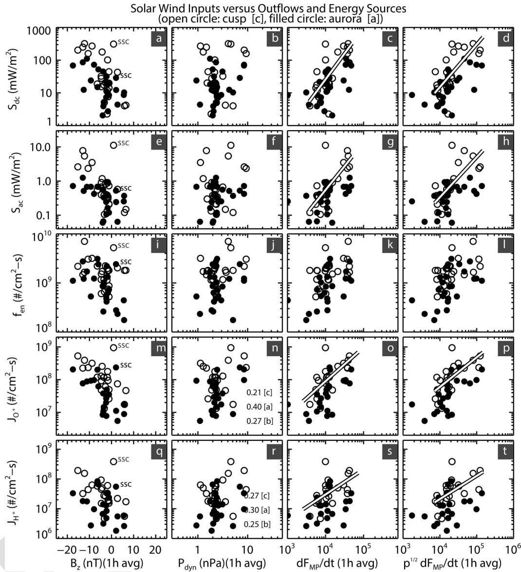
Figure 5. Scatter plots of the solar wind-magnetosphere coupling functions, B_z (leftmost column), P_{\text{dyn}} (second column from the left), d\Phi_{\text{MP}}/dt (third column from the left) and p^{1/2}d\Phi_{\text{MP}}/dt (rightmost column) versus the energy inputs, including S_{\text{dc}} , S_{\text{ac}} , and f_{\text{en}} , and the outflow fluxes, including J_{\text{O}^+} and J_{\text{H}^+} . Intensities of the particle fluxes are averaged over the time period of the dayside cusp outflow (open circle) and the nightside aurora outflow (filled circle), while the maxima of S_{\text{dc}} and S_{\text{ac}} are used. The coupling functions are the averages over one hour prior the outflows observed by FAST. Correlations are computed for the dayside cusp, the nightside aurora, and the both regions, individually. In panels (c), (d), (g), (h), (o), (p), (s), (t), the best fitting lines are added to the scatters of the solar wind coupling functions, d\Phi_{\text{MP}}/dt and p^{1/2}d\Phi_{\text{MP}}/dt versus the energy inputs and the outflows in the cusp region.
