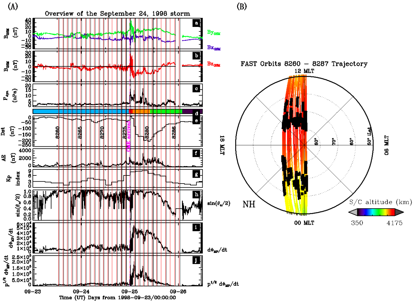
Figure 1. Left-hand plot (A): overview of the storm. From top-down, the plot shows (a) the interplanetary magnetic field Bx and By, (b) Bz, (c) the solar wind dynamic pressure, (d) the color code of the storm phase (blue for pre-storm times, dark red for the initial phase, orange for the main phase, and green for the recovery phase), (e) the Dst index, with some orbit numbers labelled at the vertical lines which indicate the start times of the dayside outflows (in red) and the nightside outflows (in black), (f) the AE index, and (g) the Kp index, (h) \sin\left(\frac{\theta_c}{2}\right) , where \theta_c is the IMF clock angle, (i) the rate magnetic flux is opened at the magnetopause, d\Phi_{MP}/dt , and (j) p^{1/2}d\Phi_{MP}/dt , where p is the solar wind dynamic pressure (Newell et al., 2007). The magenta vertical line indicates the time of the coronal mass ejection (CME) arrival. Right-hand plot (B): trajectories of the 28 FAST orbits. The coordinate system is magnetic local time by magnetic invariant latitude. The Sun is in the upward direction. The bolded segments represent the time intervals when outflows are observed in either the nightside auroral oval zone or the dayside cusp region, as Strangeway et al. (2005) did but they used 33 orbits and considered data acquired only on the dayside. The color code indicates the spacecraft altitude above the Earth's surface.
