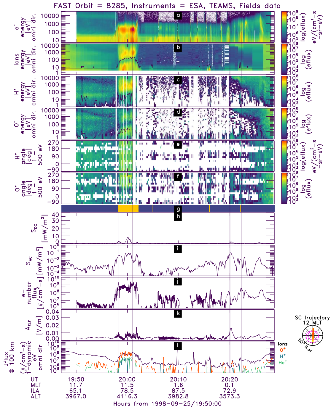
330 Figure a3. Summary plot of the orbit 8285, for which the nightside proton outflow was excluded from our analysis. The panels show the same quantities as Figure 2 in our original submission.
