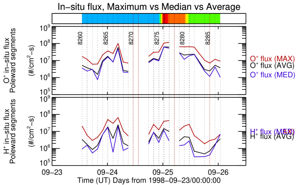
130 Figure a1. Comparison of the nightside outflow flux ( O^+ in the top panel and H^+ in the bottom panel) between the maximum (red), the median (blue) and the averaged (black) values over the outflow time periods in the nightside auroral region. Vertical red lines indicate the three orbits with large data gaps or the orbit 8285 with low flux. Orbit 8285 is included in this plot.
