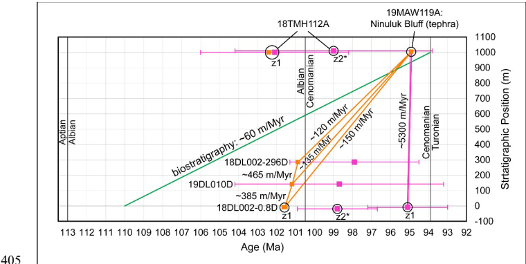
Figure 8: Age–depth plot of new and existing age constraints for the Slope Mountain stratigraphy. Data plotted in magenta and orange are laser ablation-inductively coupled plasma mass spectrometry (LA-ICPMS) and chemical abrasion-isotope dilution-
