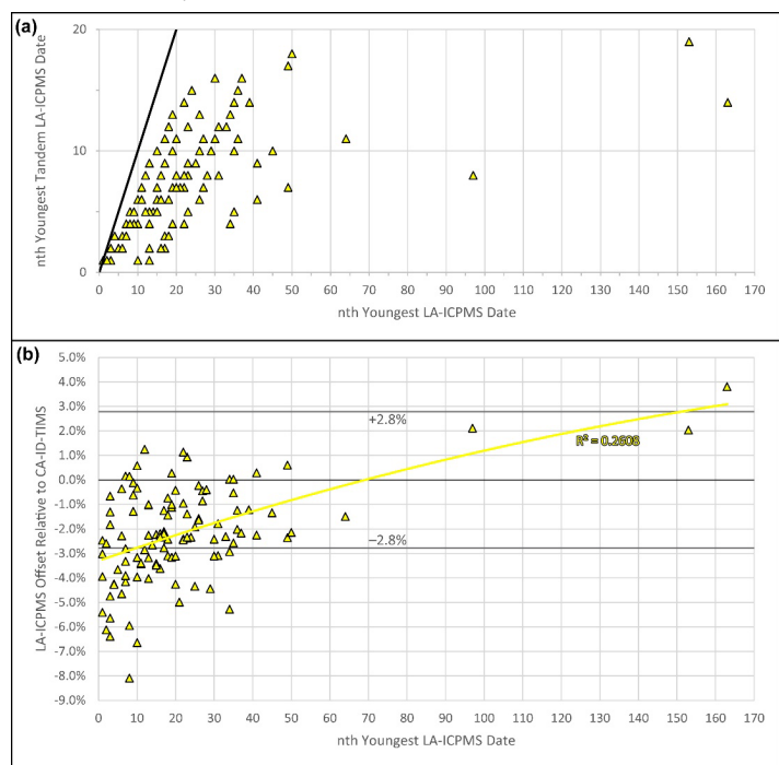
Figure 11: Plots highlighting the context of sampling somewhat broadly across laser ablation-inductively coupled plasma mass spectrometry (LA-ICPMS) date distributions for follow-up (tandem) dating by chemical abrasion-isotope dilution-thermal ionization mass spectrometry (CA-ID-TIMS). Data plotted are from Rasmussen et al. (2021), with additional date-rank context from
