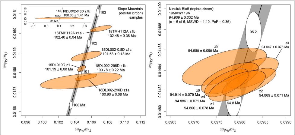
275 Figure 4: Conventional U–Pb concordia plots (Wetherill, 1956) of all chemical abrasion-isotope dilution thermal ionization mass spectrometry data for the detrital zircon results at Slope Mountain (left) and tephra zircon results at Ninuluk Bluff (right). Orange uncertainty ellipses reflect 95% confidence intervals; all z1a–z1b grain fragment pairs overlap at ratio uncertainties. Inset at upper left includes the relatively imprecise analysis from 18DL002-0.8D z1b fragment, which is excluded from the main plot at left (see text for discussion). Date uncertainties are ± 2σ (X). Plots were generated in IsoplotR (Vermeesch, 2018); gray concordia bands depict the 95% confidence interval associated with uranium decay constants and 238 U/ 235 U ratio. See Herriott et al. (2024) for complete data tables.
